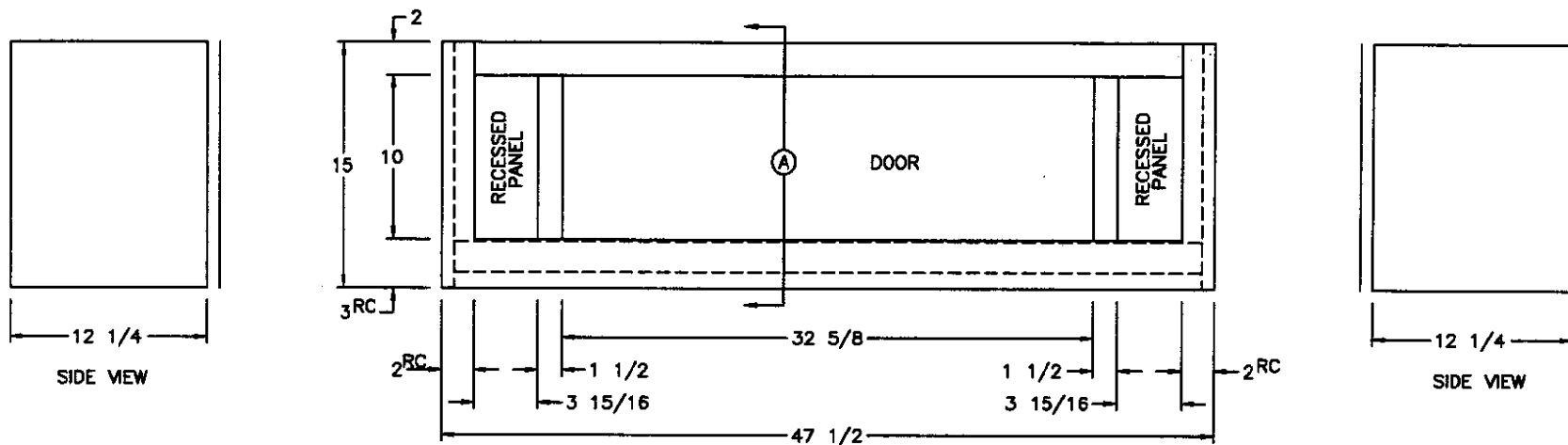
FRONT VIEW (2) 16 1/2x11 1/2 GLASS DOORS
