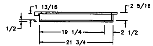
SIDE SECTION
