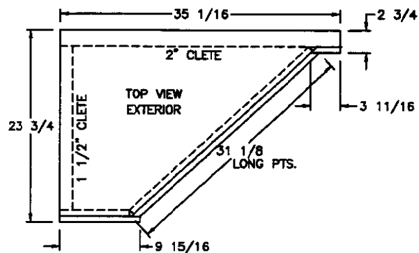
OFFDOOR SIDE
