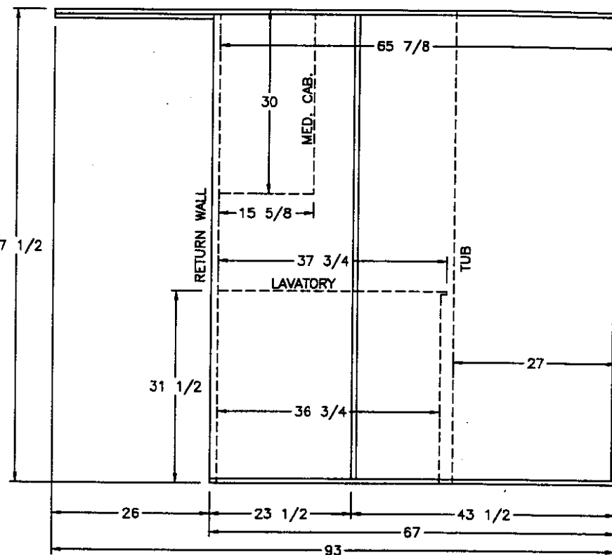
VIEW (B)
