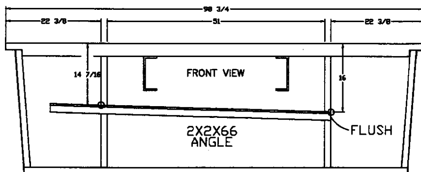
REAR HOLDING TANK CROSSMEMBER
