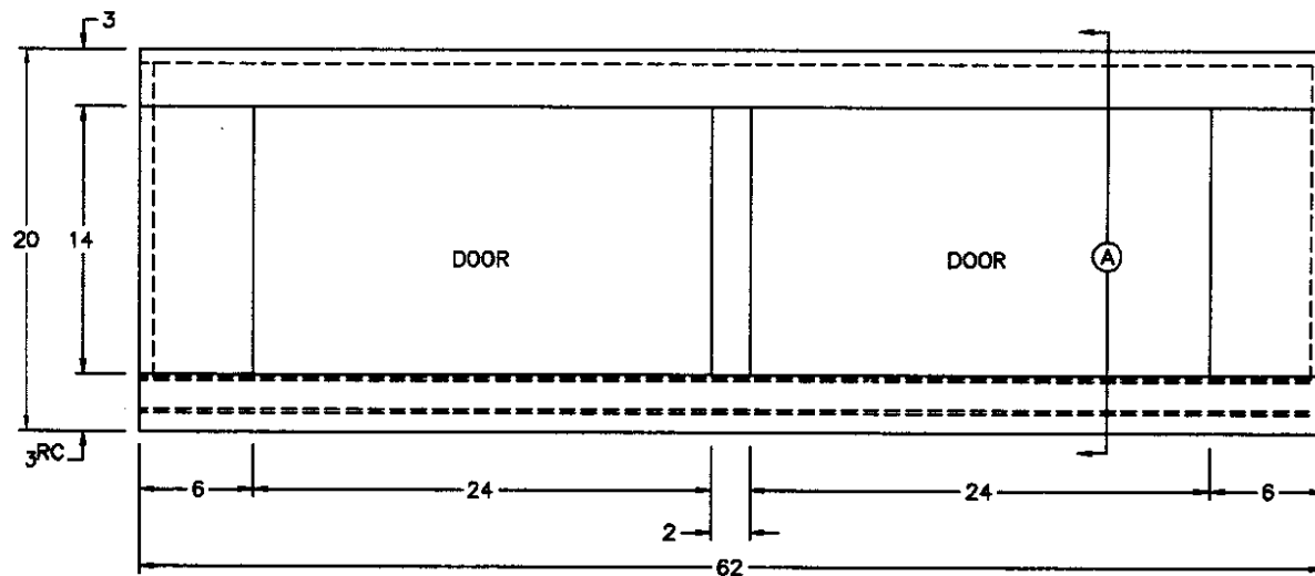
FRONT VIEW
