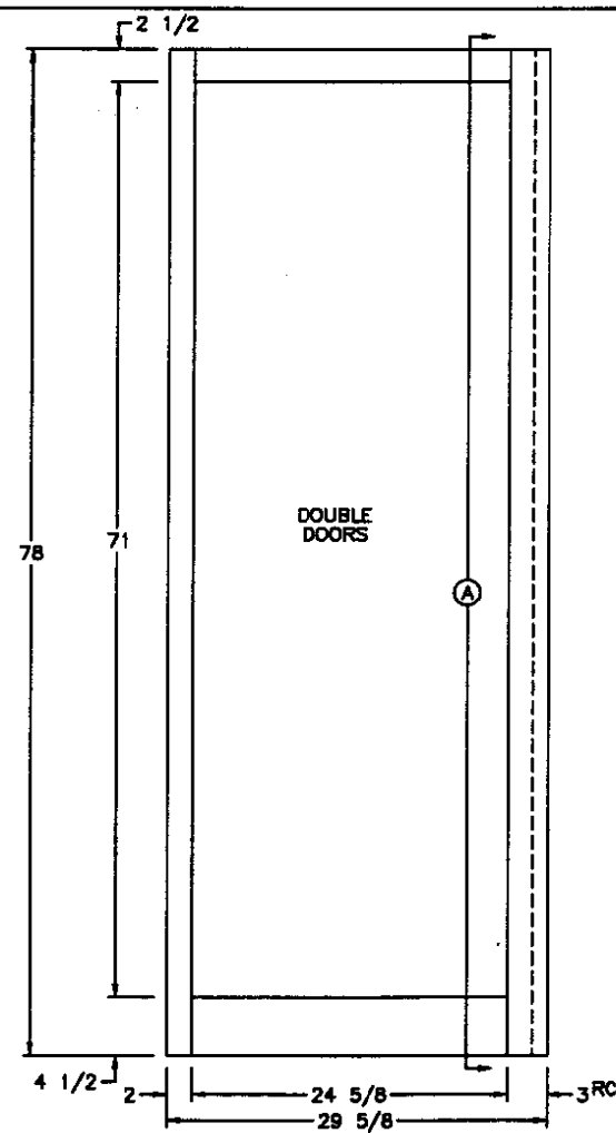
FRONT VIEW
