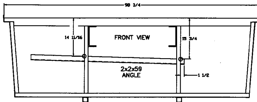
FRONT HOLDING TANK CROSSMEMBER
