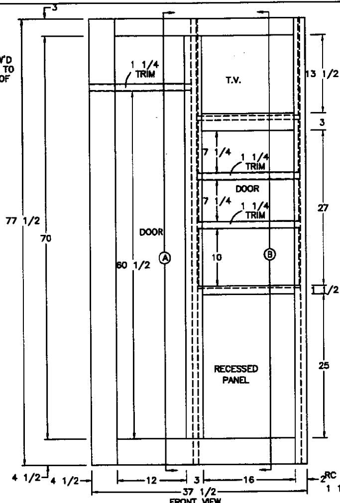
FRONT VIEW (1) 12 1/2x71 1/2 MIRROR DOOR (1) 16 1/2x27 1/2 DOOR
