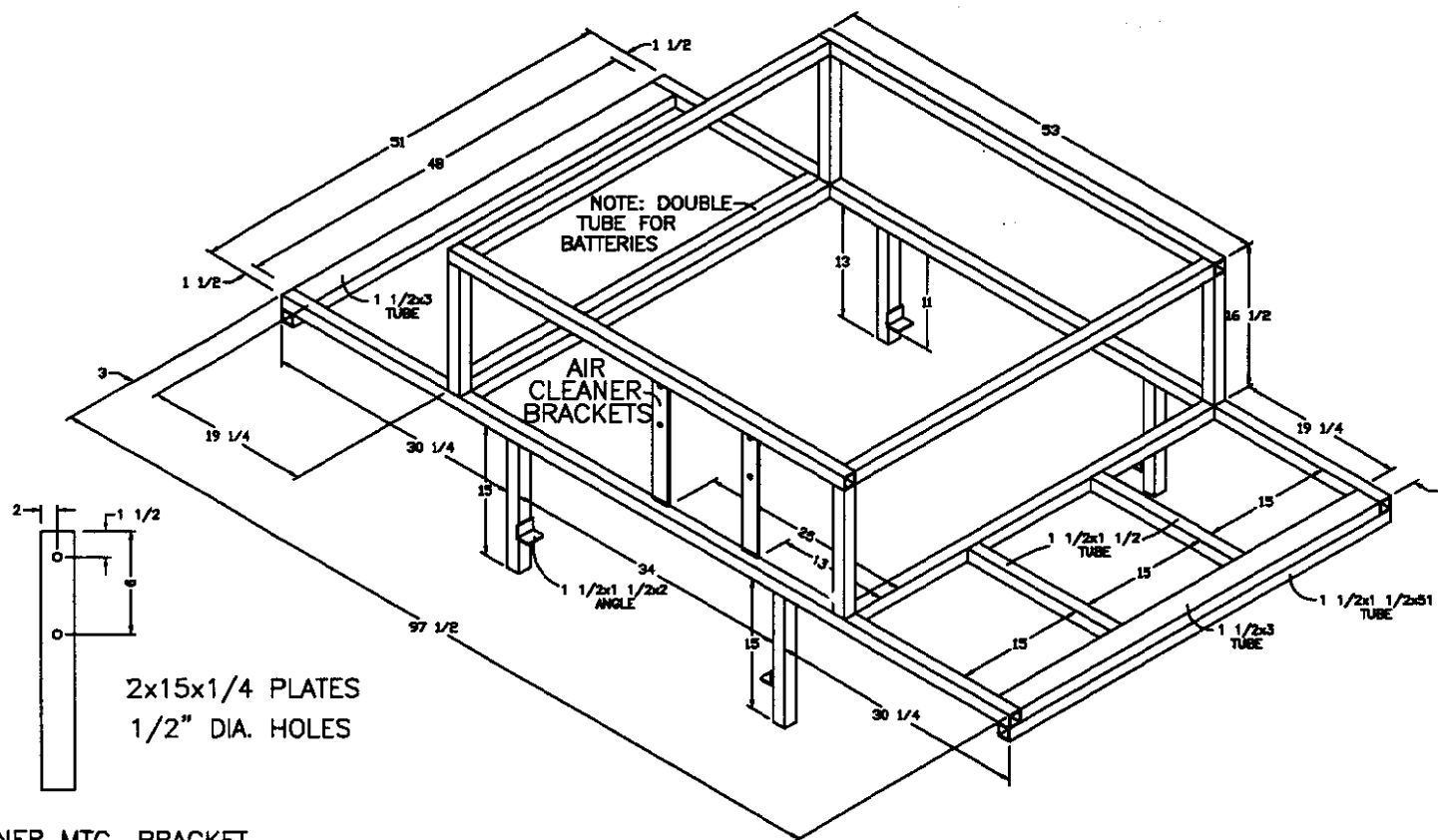
AIR CLEANER MTG. BRACKET
