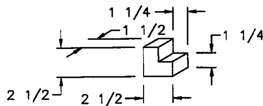
WALL BLOCK FOR WATER LINES TWO PER UNIT REQ'D
