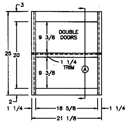
FRONTS (2) 9 1/2x20 1/2 DOORS
