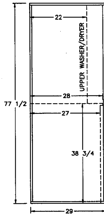
VIEW ⑤
