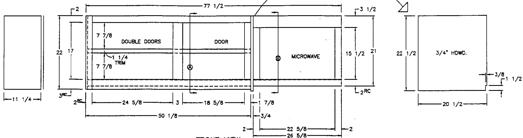
FRONT VIEW (2) 12 1/2x18 1/2 DOORS (2) 9 1/2x18 1/2 DOORS
