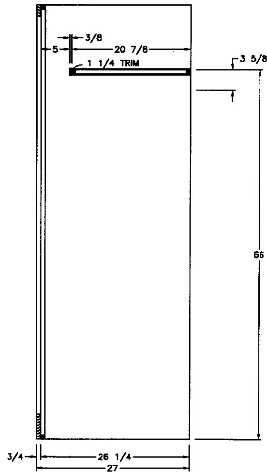
SIDE SECTION (A)
