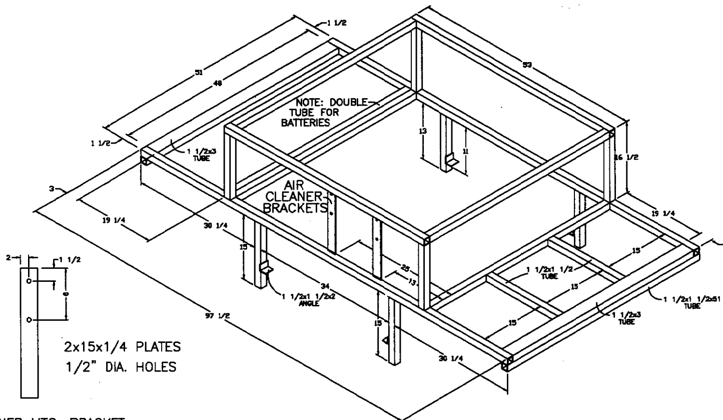
AIR CLEANER MTG. BRACKET
