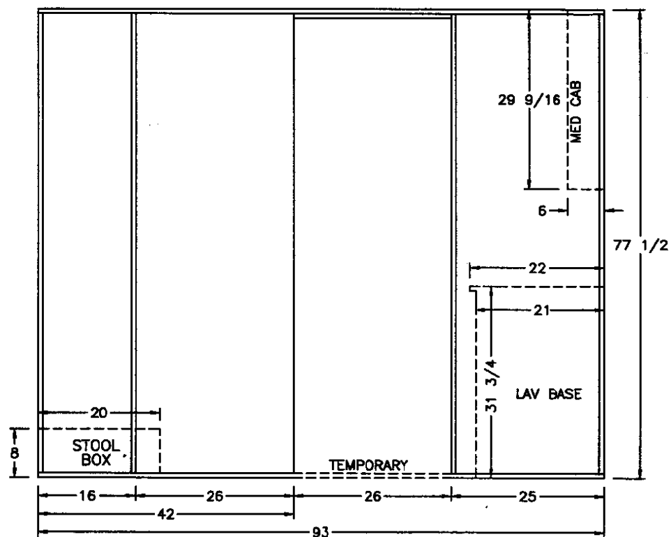
VIEW (B)
