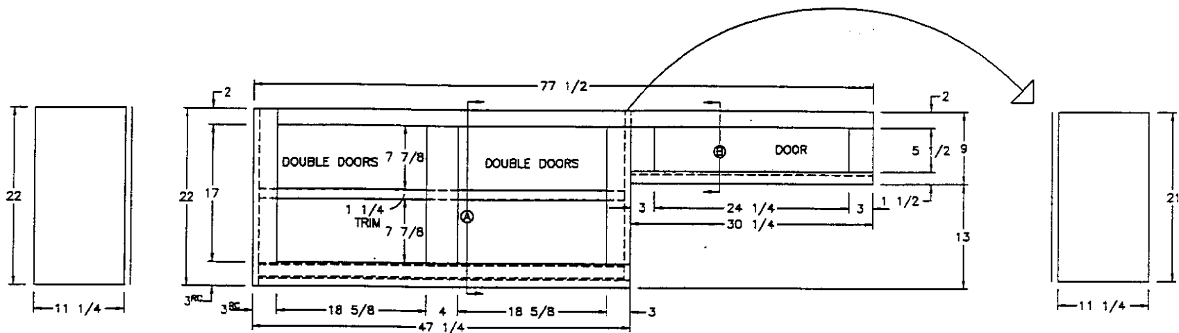
FRONT VIEW
