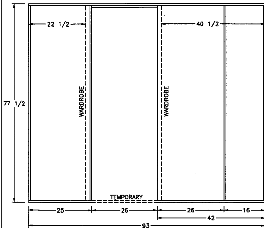
VIEW (A)
