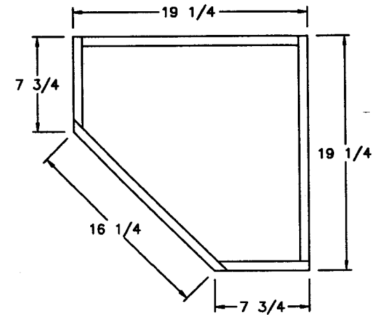
BOTTOM PANEL
