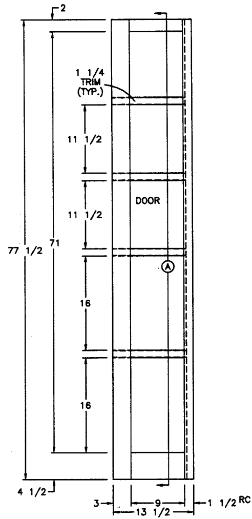
FRONT VIEW
