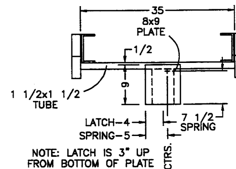
REAR END VIEW
