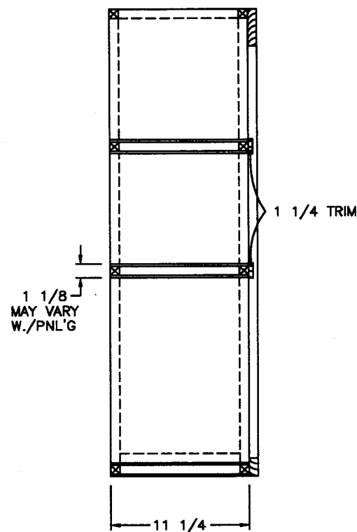
SIDE SECTION (A)
