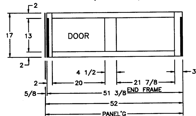
END (INTERIOR VIEW)
