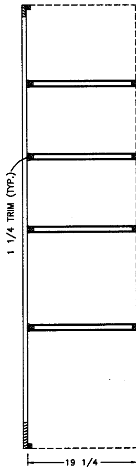
SIDE SECTION (A)
