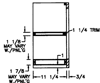
SIDE SECTION (A)
