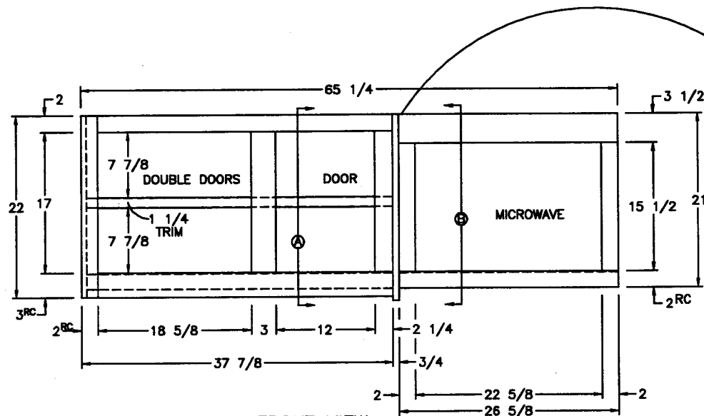
FRONT VIEW (2) 9 1/2x18 1/2 DOORS (1) 12 1/2x18 1/2 DOORS
