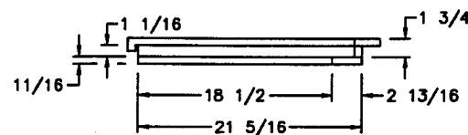
SIDE SECTION
