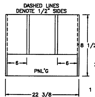
DETAIL C - BOTTOM 1/2" PLYW'D
