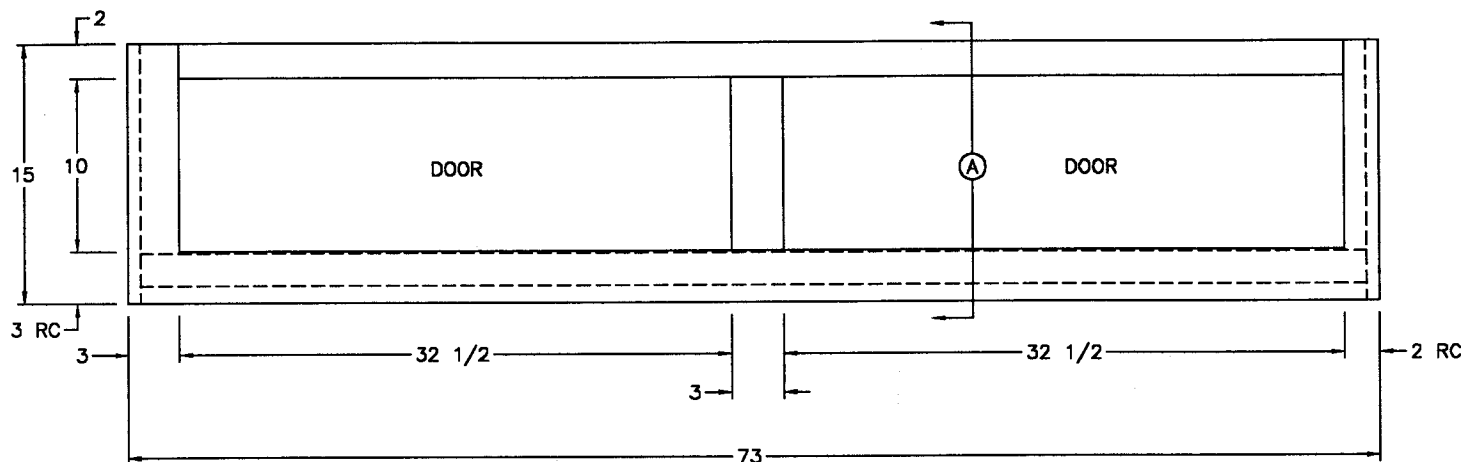
FRONT VIEW (4) 16 1/2x11 1/2 GLASS DOORS
