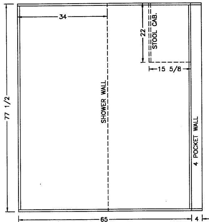
VIEW (E)
