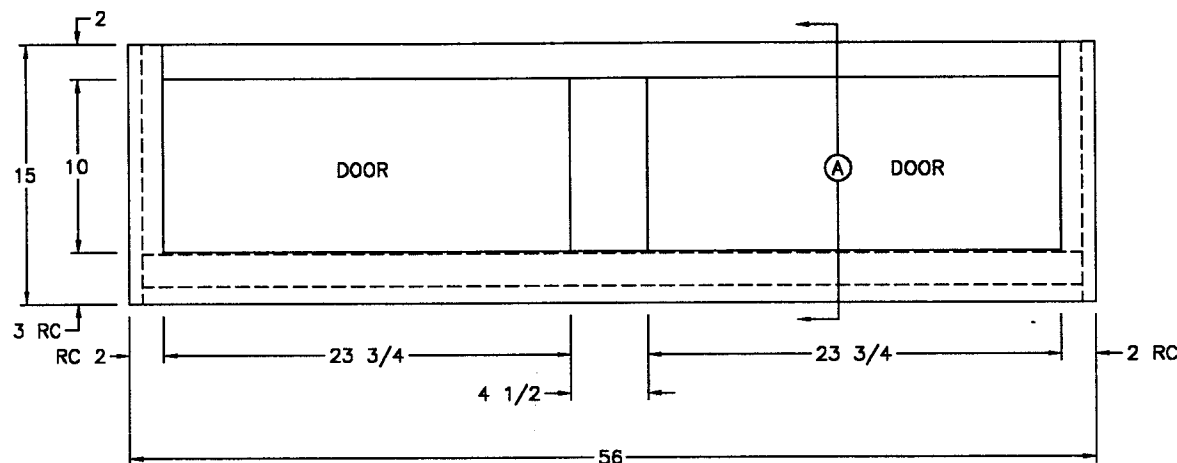
FRONT VIEW (2) 24 1/2x11 1/2 DOORS
