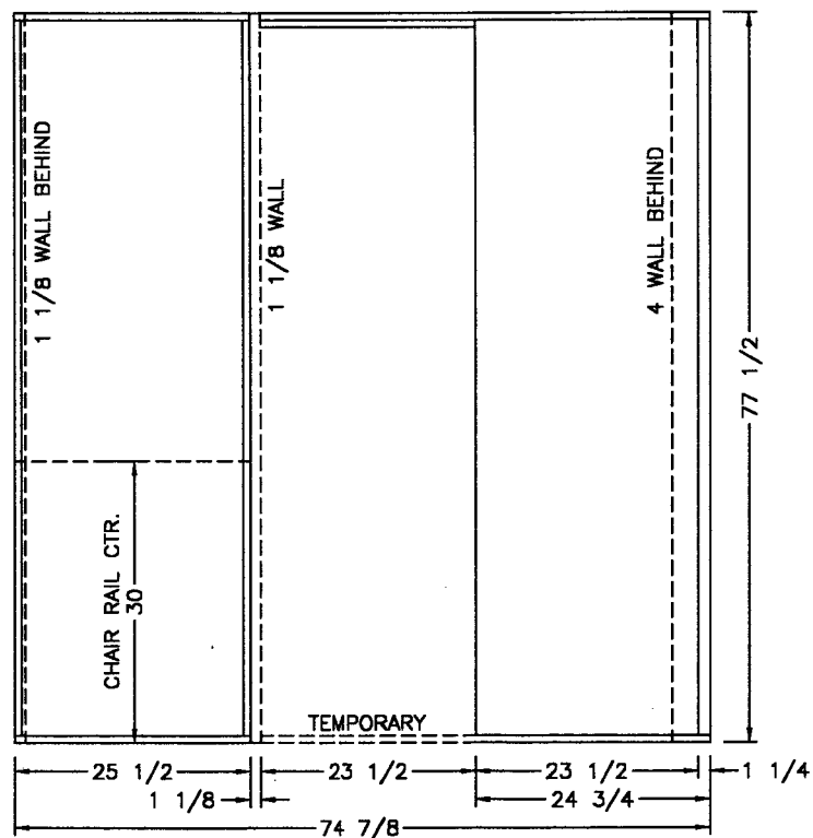
VIEW C
