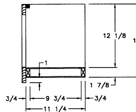
SIDE SECTION A
