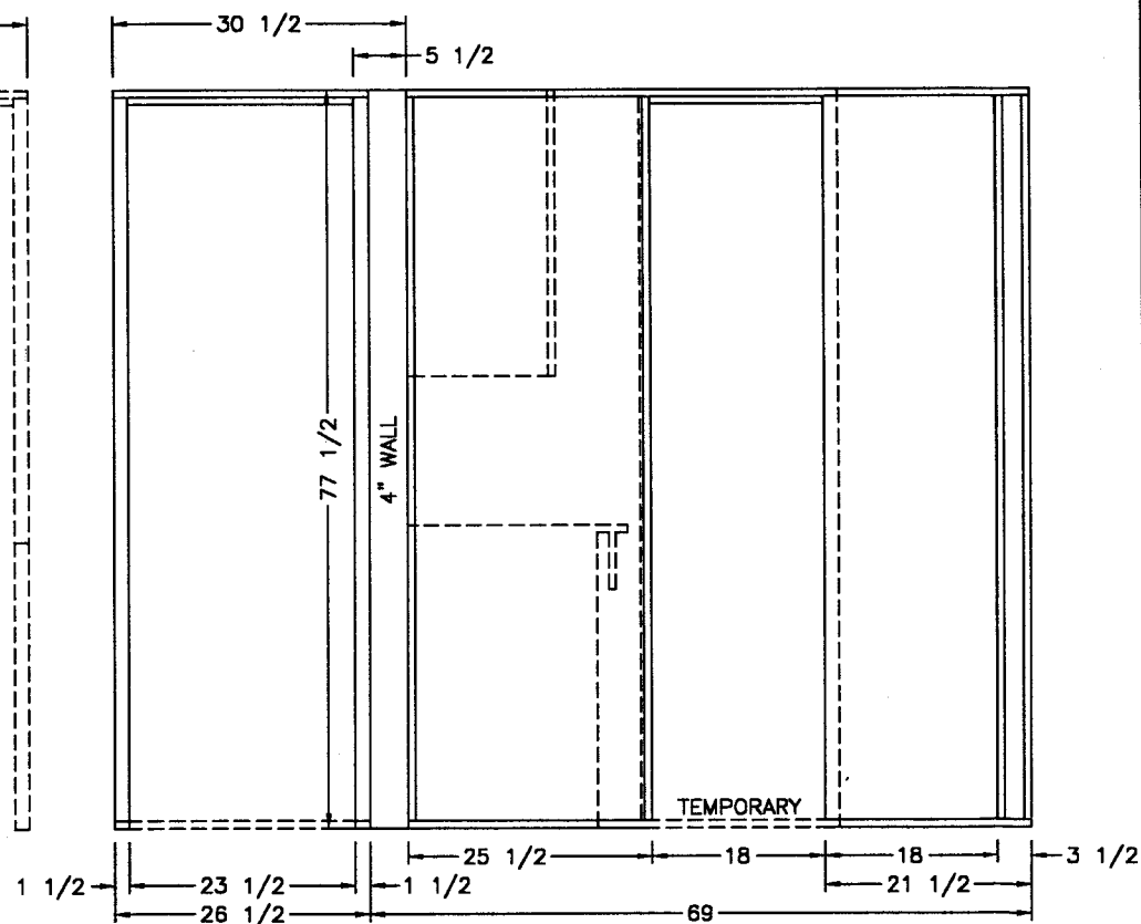
VIEW (B)
