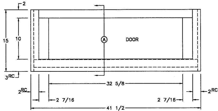
FRONT VIEW (2) 16 1/2x11 1/2 GLASS DOORS
