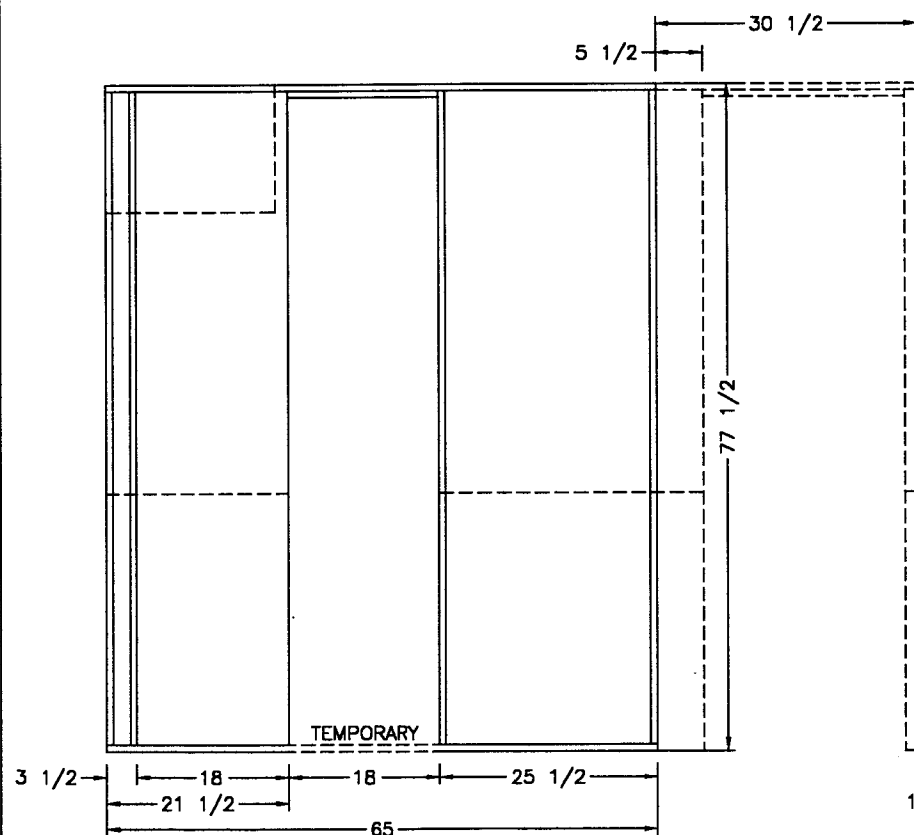
VIEW (A)
