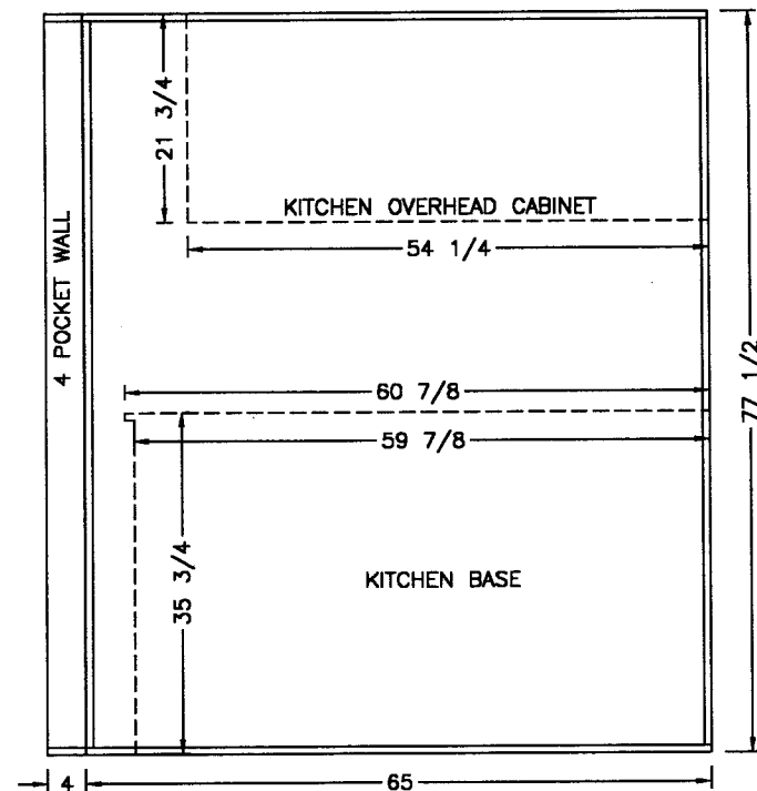
VIEW (F)
