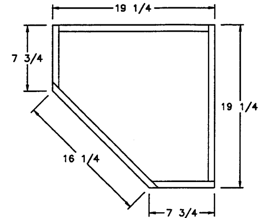
BOTTOM PANEL
