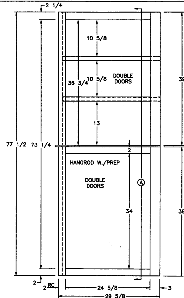
FRONT VIEW
