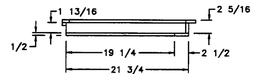
SIDE SECTION
