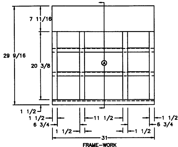
DECORATIVE WALL PANEL TOP BETWEEN MIRROR FRAME & CEILING
