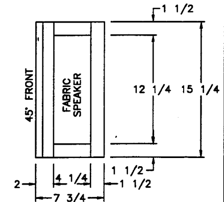
RT END VIEW
