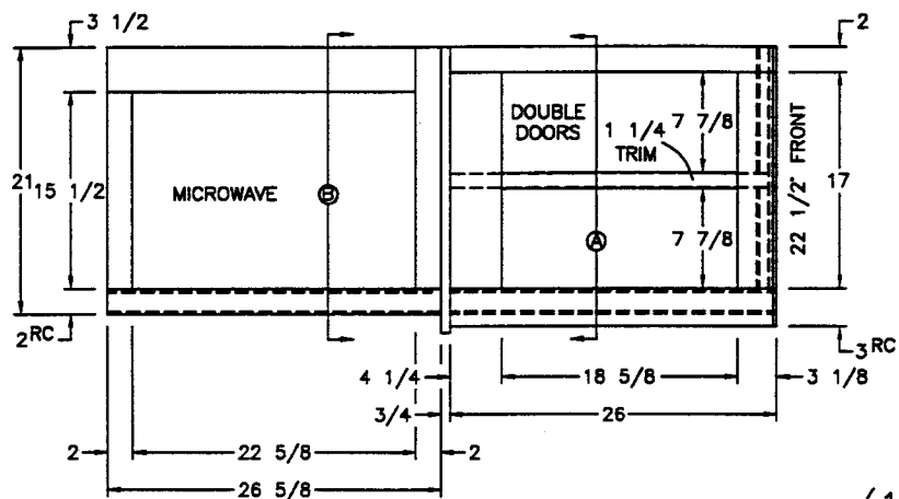
(2) 9 1/2x18 1/2 DOORS
