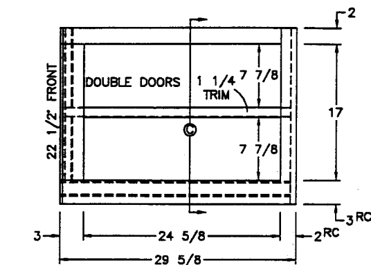
(2) 12 1/2x18 1/2 DOORS
