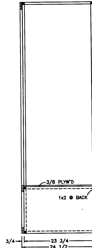
SIDE SECTION (A)
