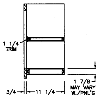
SIDE SECTION (A)
