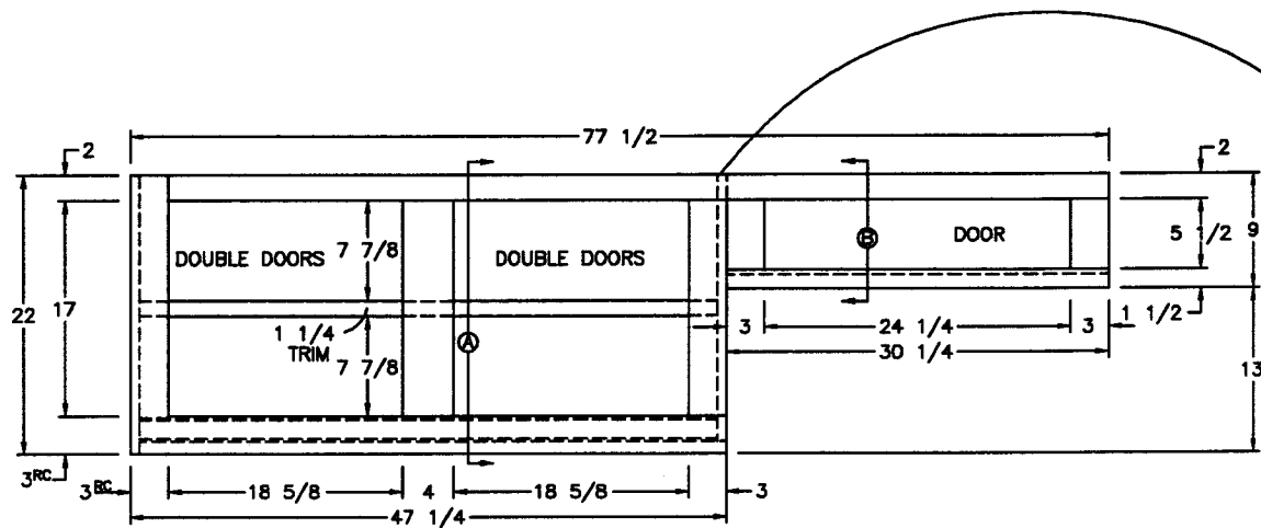
FRONT VIEW
