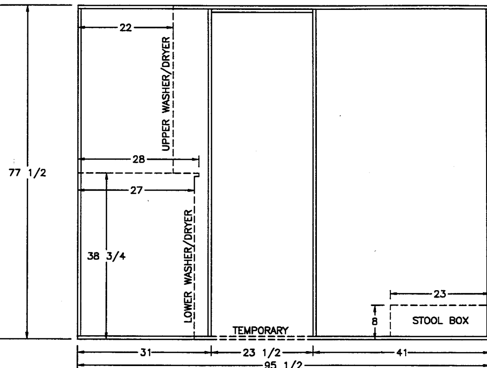
VIEW (B)
