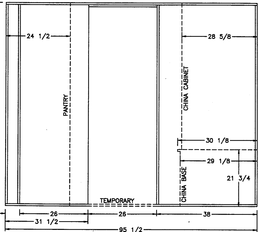
VIEW D
