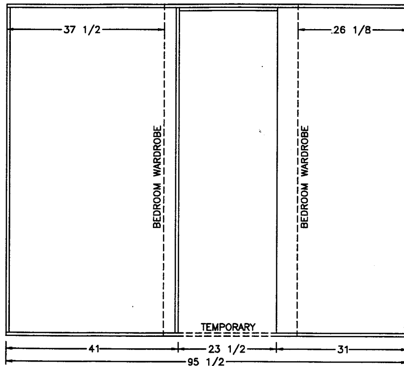
VIEW (A)
