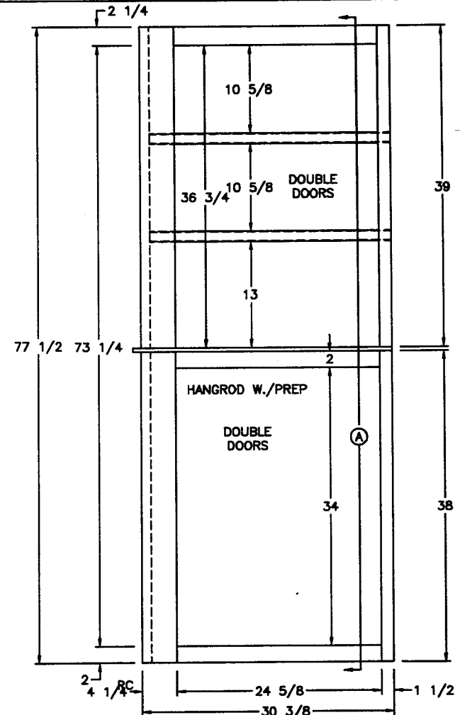
FRONT VIEW
