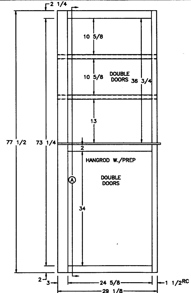
FRONT VIEW
