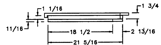
SIDE SECTION
