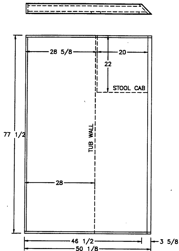
VIEW C
