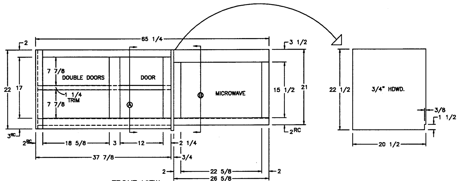
FRONT VIEW (2) 9 1/2x18 1/2 DOORS (1) 12 1/2x18 1/2 DOORS
