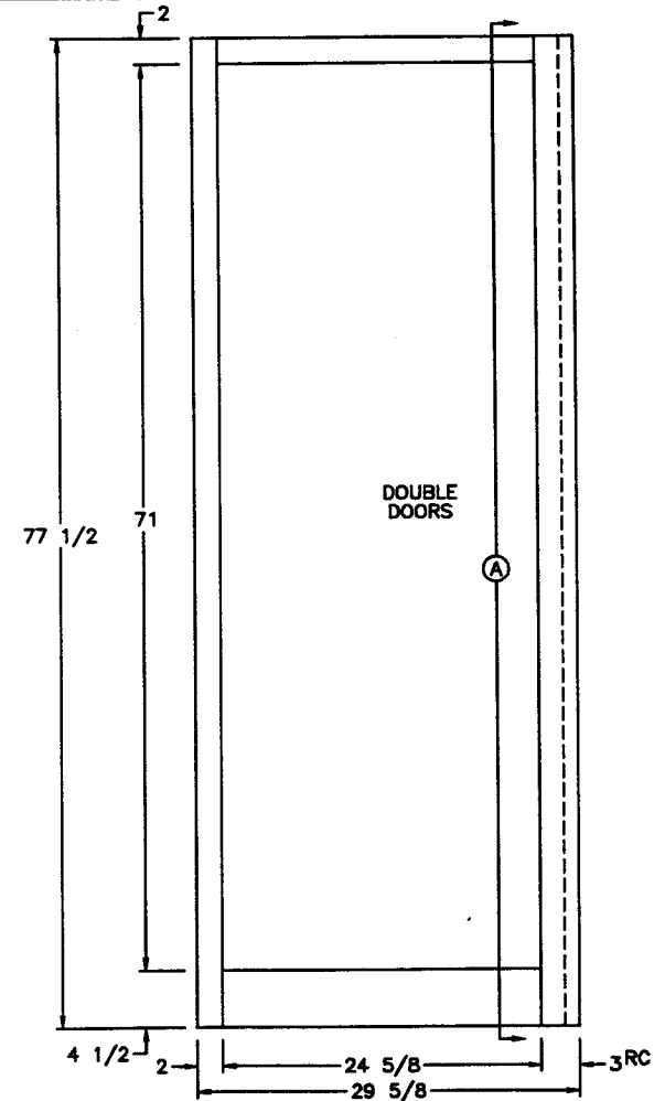
FRONT VIEW
