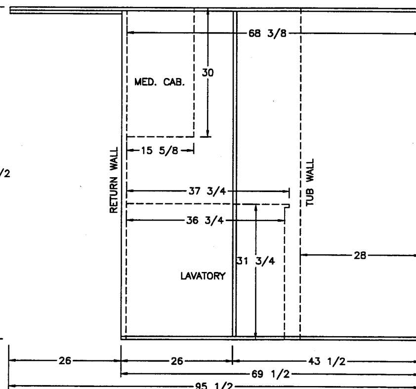
VIEW (B)
