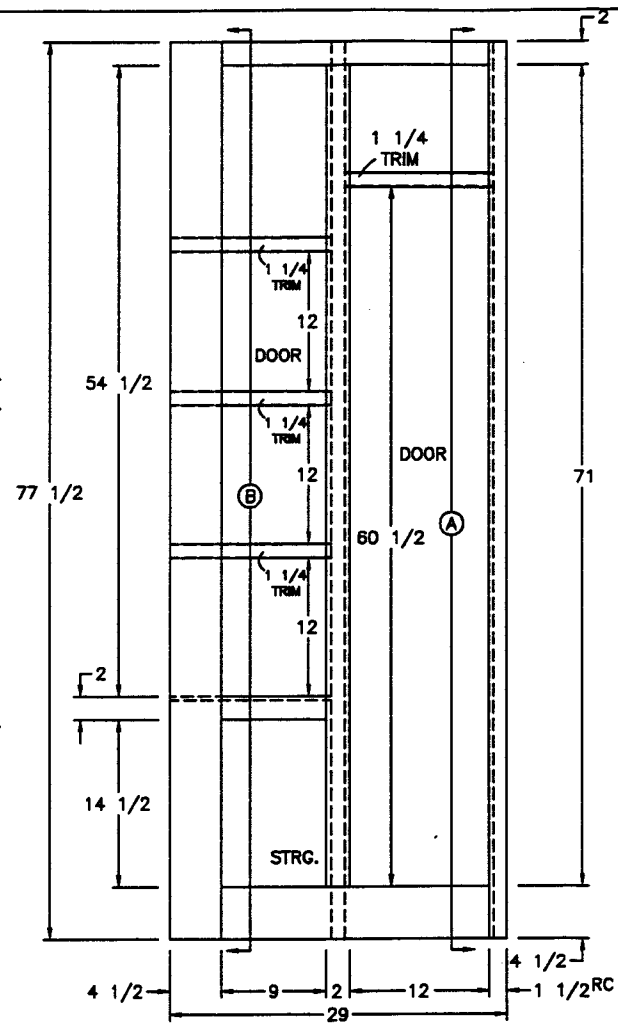
FRONT VIEW
