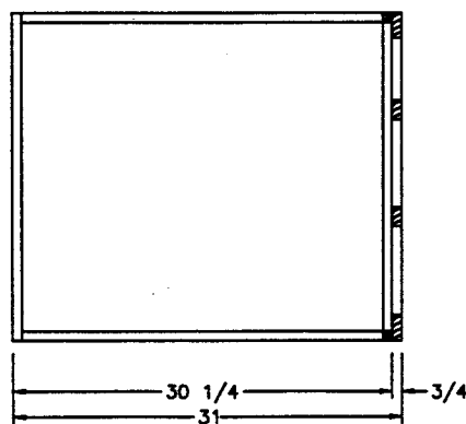
SIDE SECTION (A)
