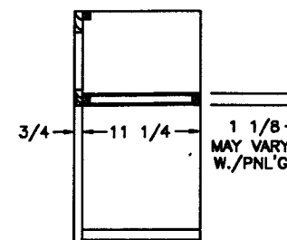
SIDE SECTION (B)
