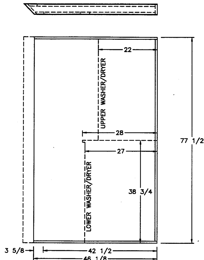
VIEW D
