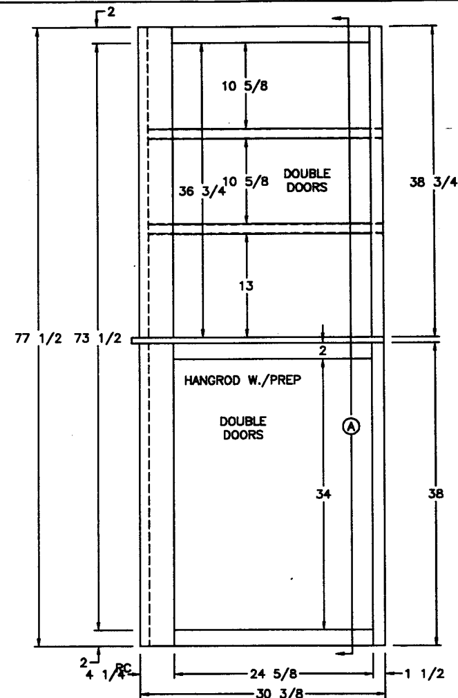
FRONT VIEW
