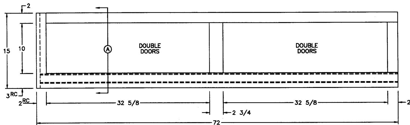
FRONT VIEW (4) 16 1/2x11 1/2 DOORS
