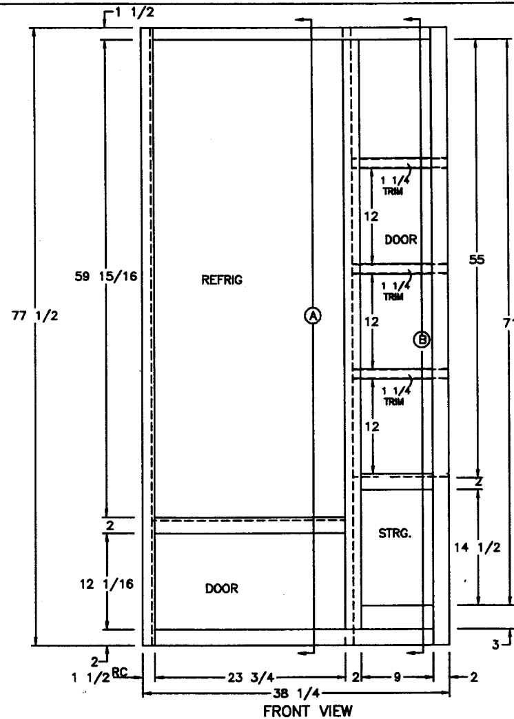
FRONT VIEW
