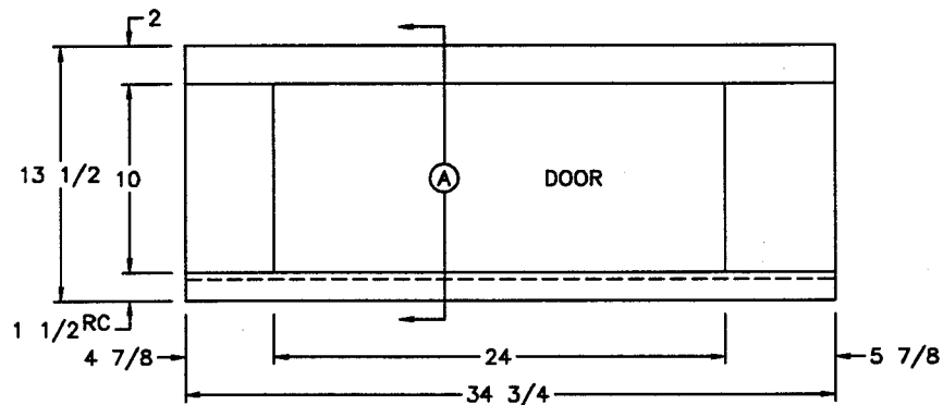
FRONT VIEW
