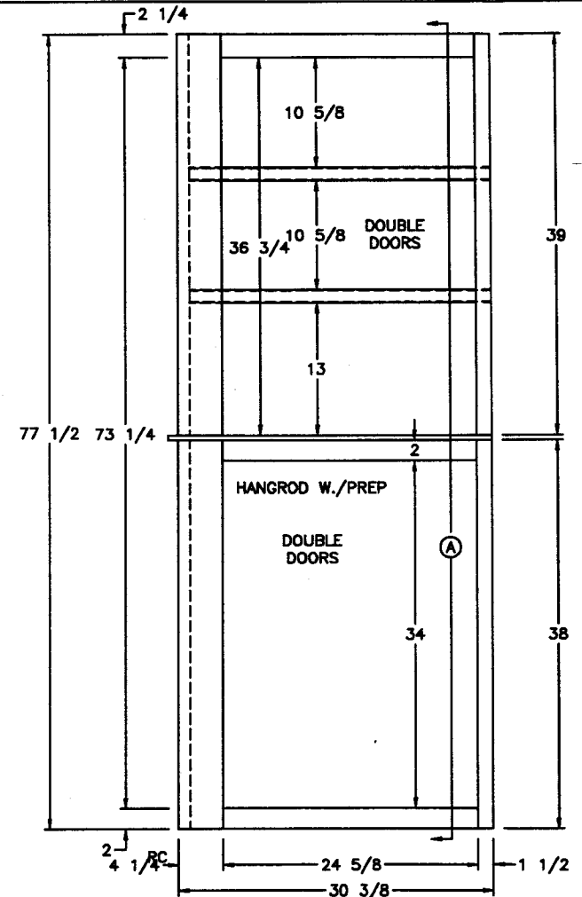
FRONT VIEW (A)
