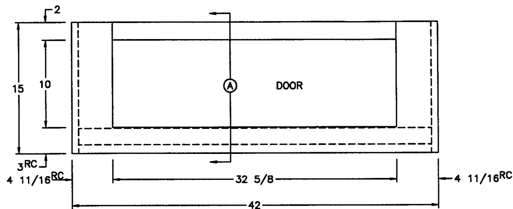
FRONT VIEW (2) 16 1/2x11 1/2 GLASS DOORS
