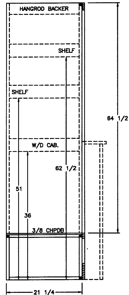
SIDE SECTION (B)
