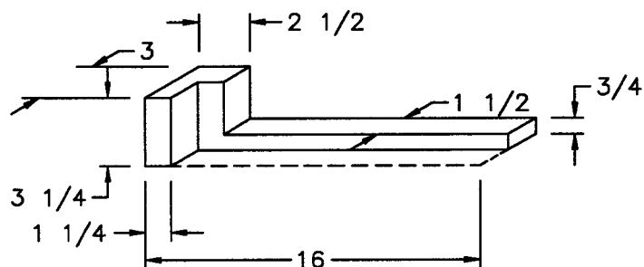
FLOOR BLOCK FOR WATER AND DRAIN LINES ONE PER UNIT REQ'D
