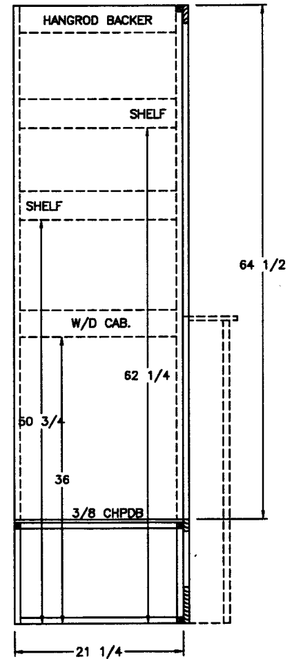
SIDE SECTION (B)
