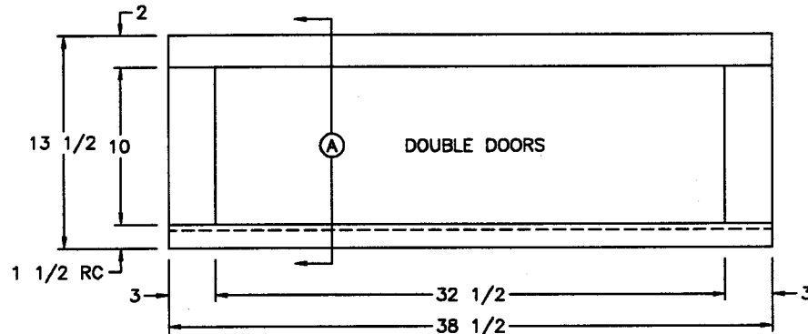
FRONT VIEW (2) 16 1/2x10 1/2 DOORS
