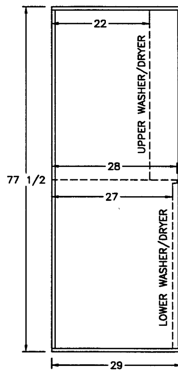
VIEW E
