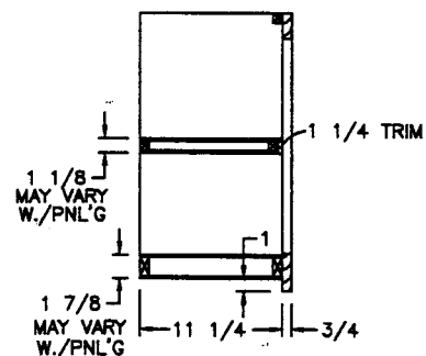
SIDE SECTION (A)
