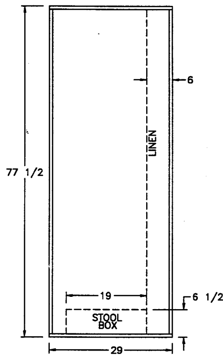
VIEW D
