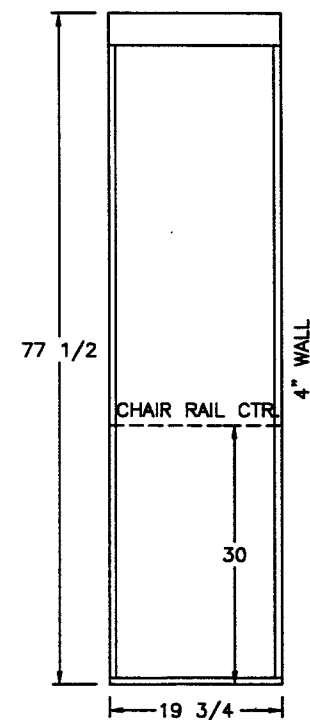
VIEW F
