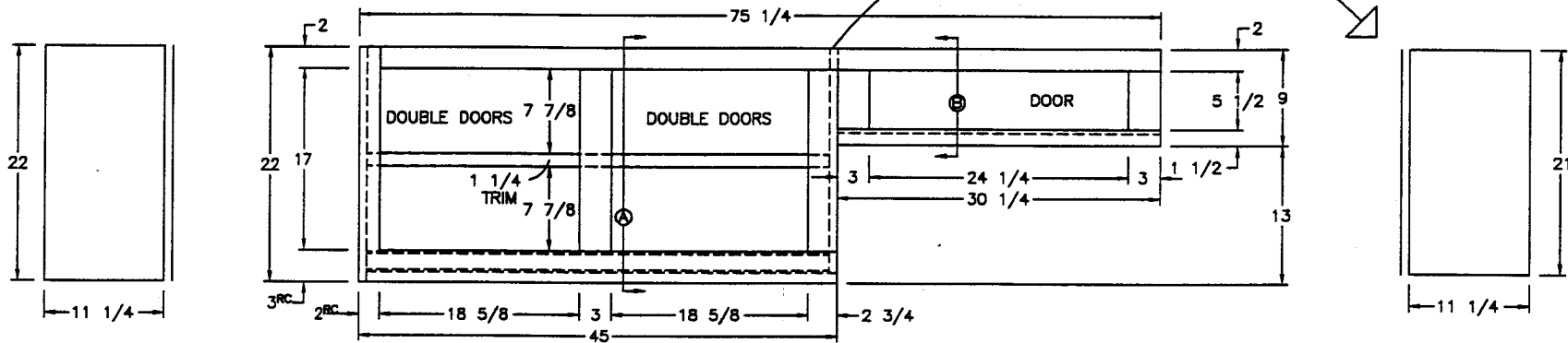
FRONT VIEW
