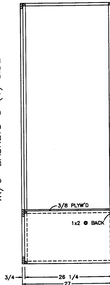
SIDE SECTION (A)
