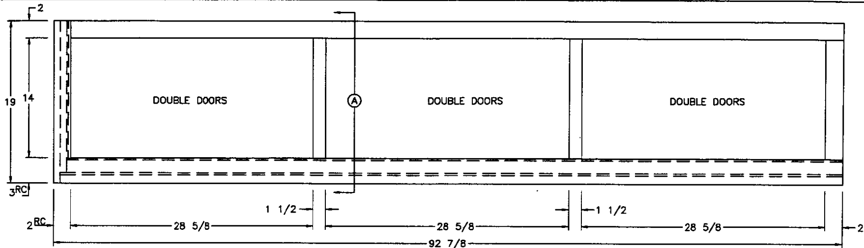
FRONT VIEW (6) 14 1/2x15 1/2 DOORS
