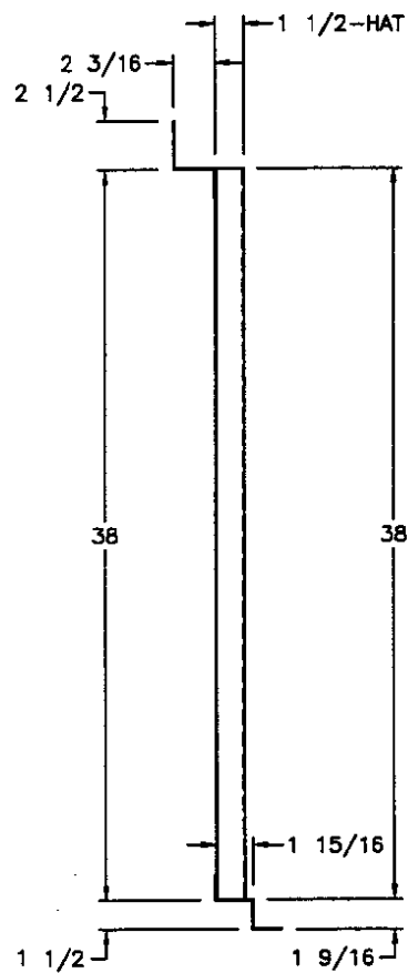
SIDE PROFILE (A)
