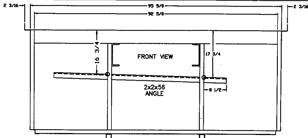
FRONT HOLDING TANK CROSSMEMBER
