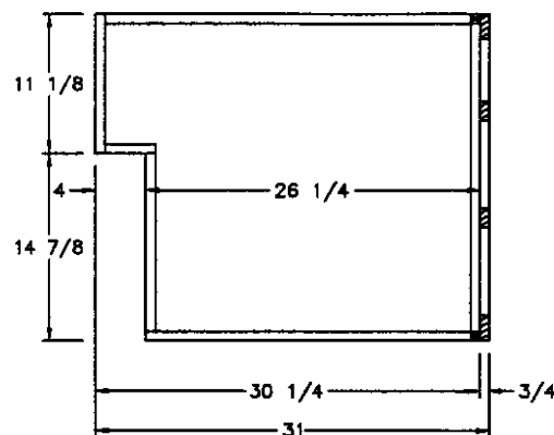
SIDE SECTION (A)
