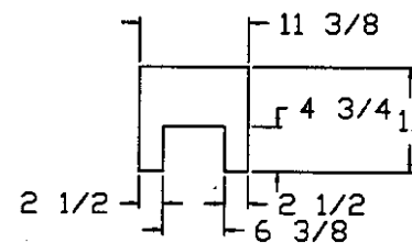
Plywood detail
