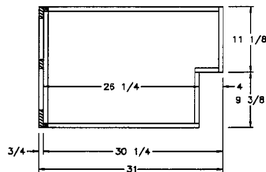
SIDE SECTION (B)
