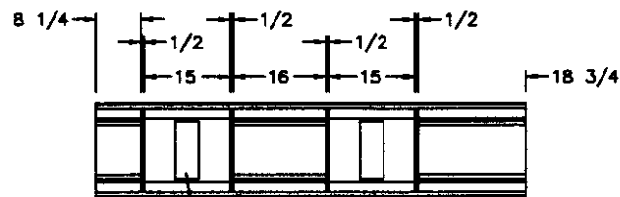
4 1/8x10 CENTERED (TYP) View from top looking down
