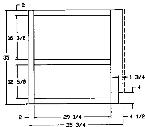
RETURN BANAK FRAME COVERED W./1/4" VENEER
