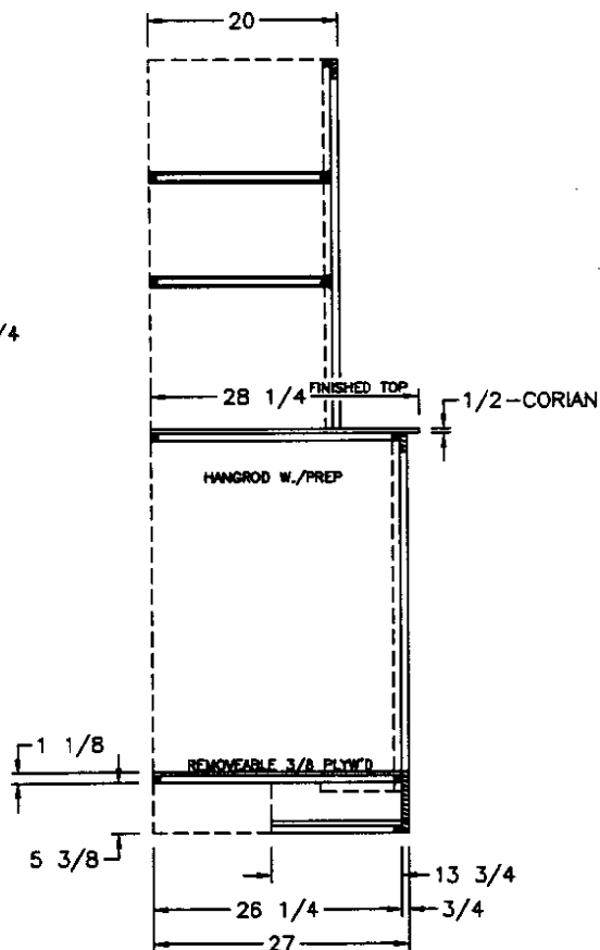
SIDE SECTION A
