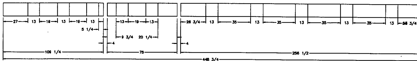
Location of 13" air slots in raceway
