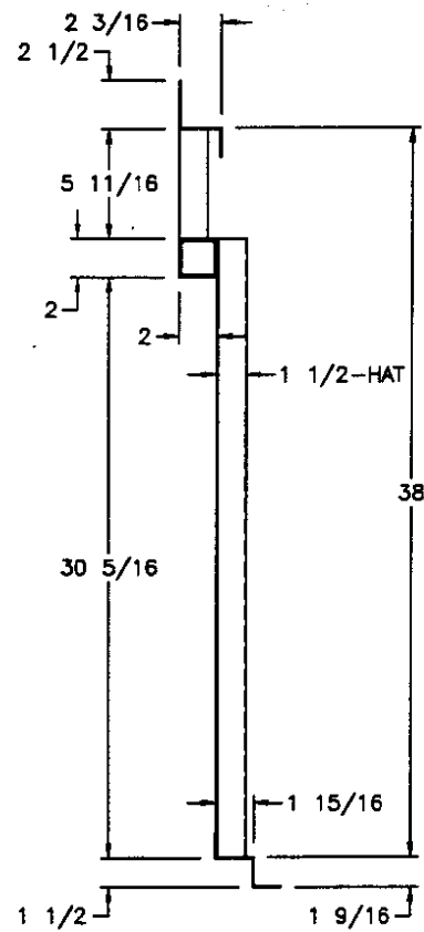
SIDE PROFILE (B)
