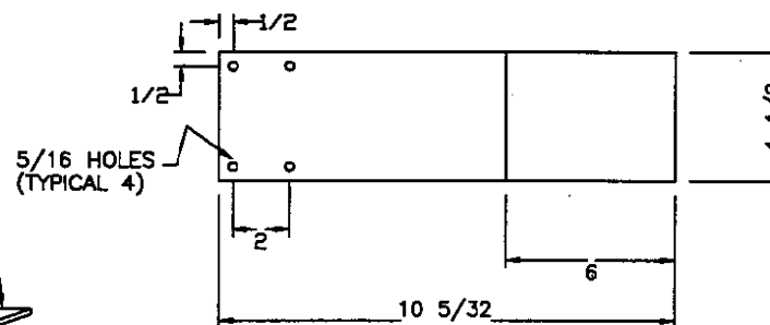
FLAT VIEW (4 1/2 X 10 5/32 X 11 GA. STEEL 2 PIECES)
