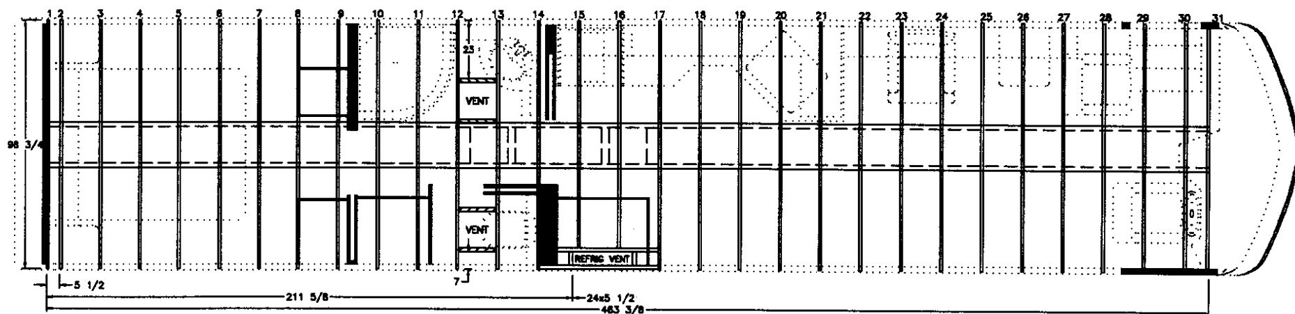
Location of 13" air slots in raceway
