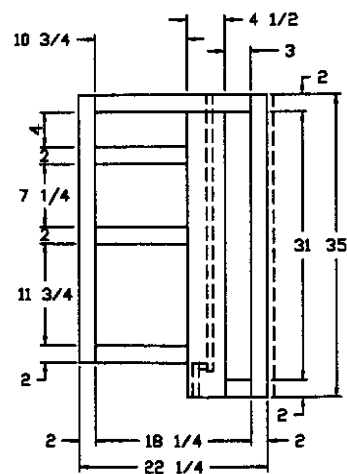
RETURN PANEL BANAK FRAME COVERED W./1/4" VENEER
