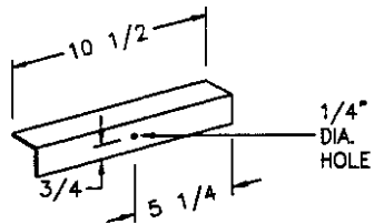
FRONT STEP PLATE ANGLE 1 1/2" X 1 1/2" X 10 1/2" FORMED ANGLE
