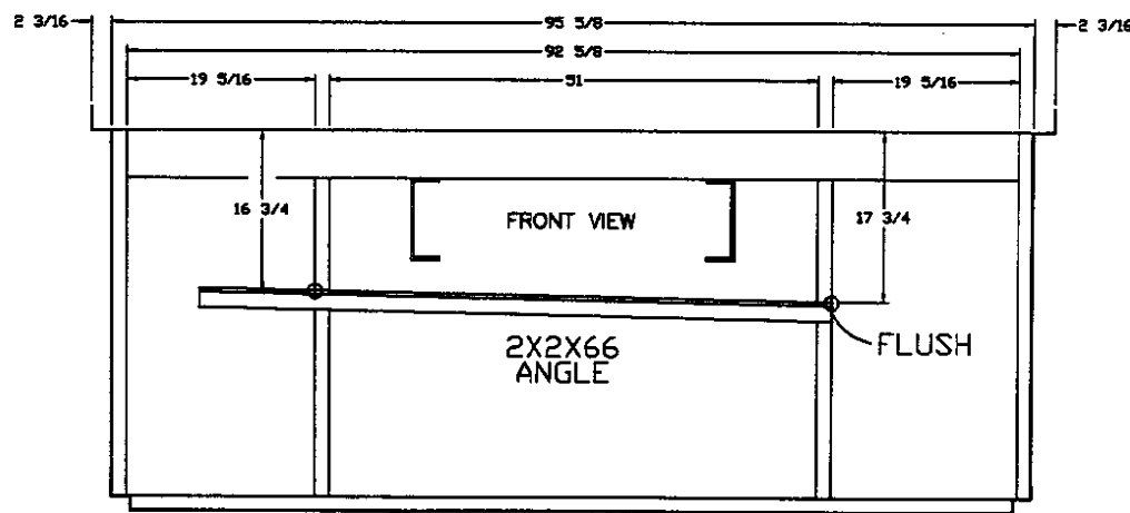
REAR HOLDING TANK CROSSMEMBER
