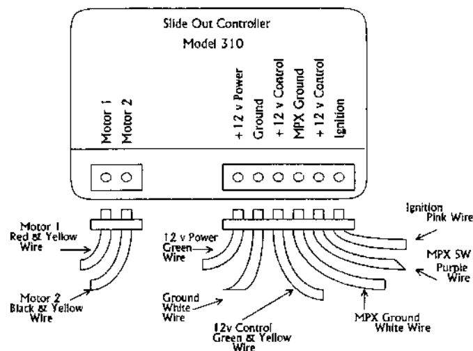
SLIDE OUT CONTROL BOX
