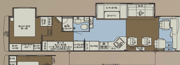
ATME 4159: Length: 41' 8" Width: 101.5"
