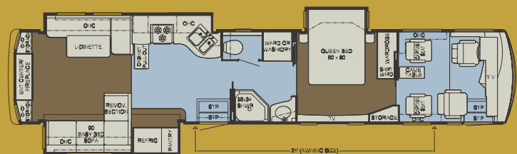
ATME 4484: Length: 44' 9" Width: 101.5"
