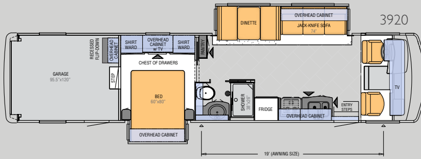
TOY HAULER FLOOR PLAN Most toy haulers don’t offer a fixed queen size bed like Canyon Star.
