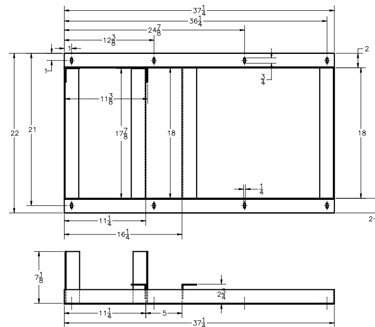
BASE ASSEMBLY 2X2 ANGLES ITEM-7
