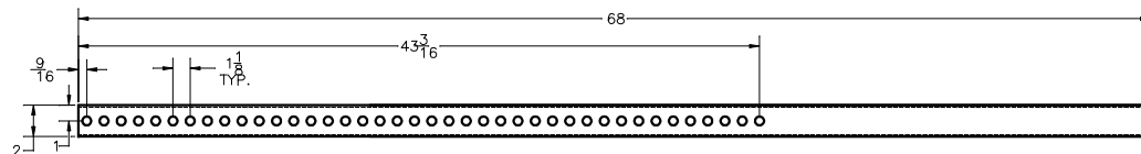
INNER TUBE ITEM-12
