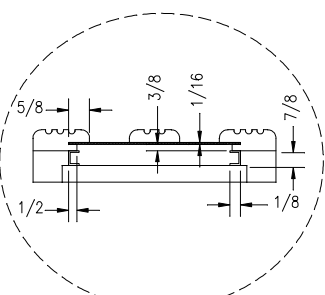
VERTICAL FASCIA DETAIL SECTION A-A SCALE: x4
