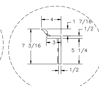
HORIZONTAL FASCIA DETAIL SECTION D-D SCALE: x2
