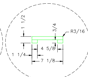
FOOT BLOCK DETAIL SECTION B-B SCALE: x2
