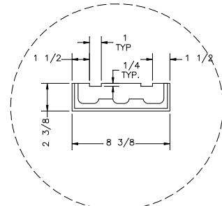
FOOT BLOCK CAP DETAIL SECTION F-F SCALE: x2
