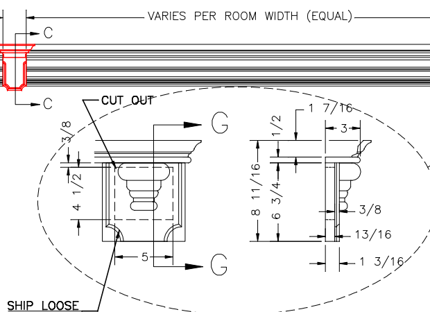
CAP BLOCK DETAIL SECTION G-G SCALE: x2
