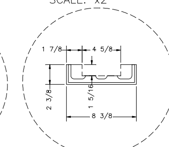
FOOT BLOCK CAP DETAIL SECTION E-E SCALE: x2
