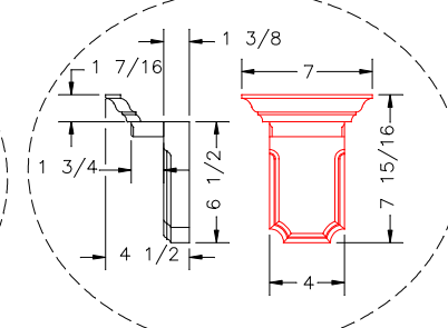
CENTER BLOCK DETAIL SECTION C-C SCALE: x2
