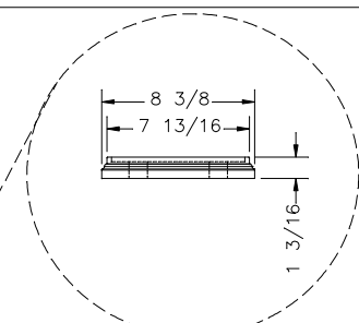
FOOT BLOCK CAP DETAIL SCALE: x2
