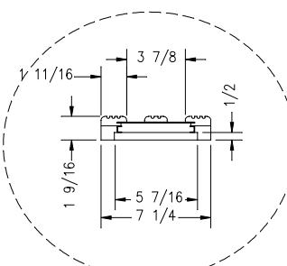
VERTICAL FASCIA DETAIL SECTION A-A SCALE: x2
