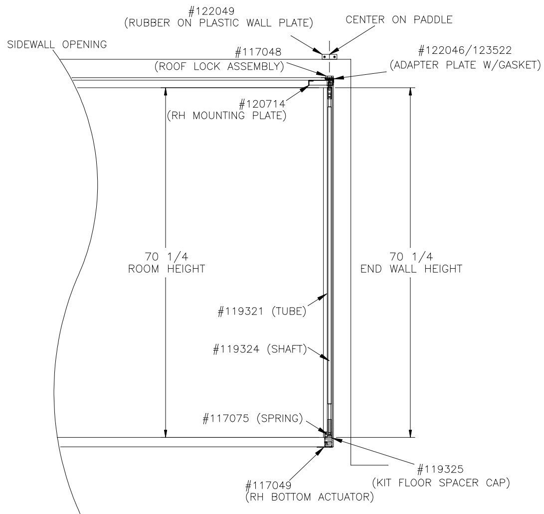
KITCHEN (RAISED)
