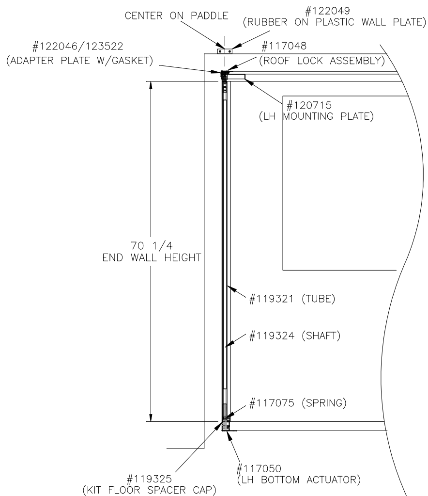
KITCHEN (RAISED)
