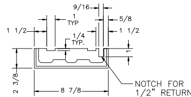
FOOT BLOCK CAP DETAIL SECTION F-F SCALE: X2
