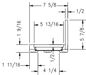
VERTICAL FASCIA DETAIL SECTION A-A SCALE: X2
