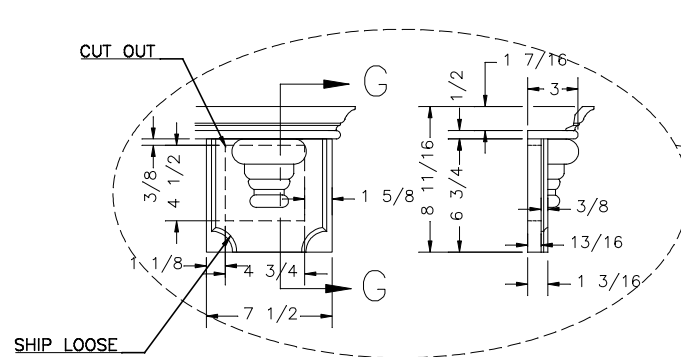
CAP BLOCK DETAIL SECTION G-G SCALE: X2
