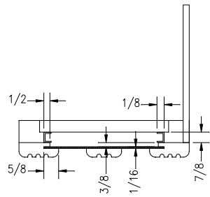
VERTICAL FASCIA DETAIL SECTION A-A SCALE: X2
