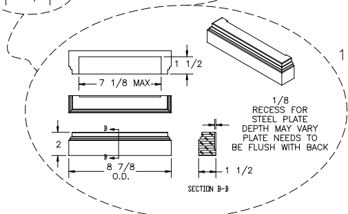
TOOL ACCESS BASE BOARD COVER DETAIL (REMOVABLE - ATTACHED WITH MAGNETS) SCALE: X2
