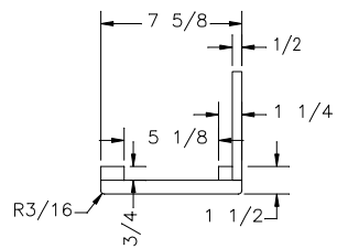
FOOT BLOCK CAP DETAIL SECTION B-B SCALE: X2
