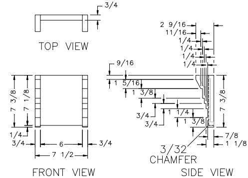
FULL WALL DIVIDER PIECE
