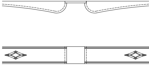
TYPICAL POCKET DOOR JAM CONFIGURATION
