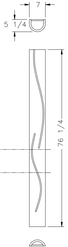
TYPICAL COLUMN
