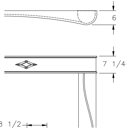
TYPICAL END LEG CONFIGURATION
