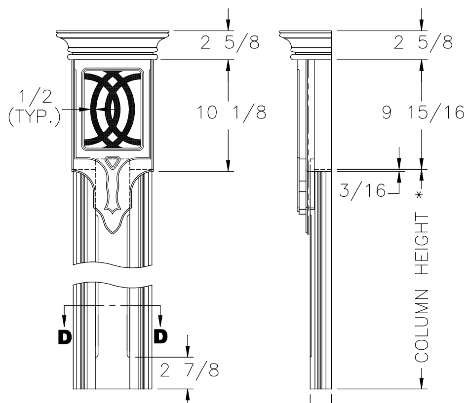
FRONT
