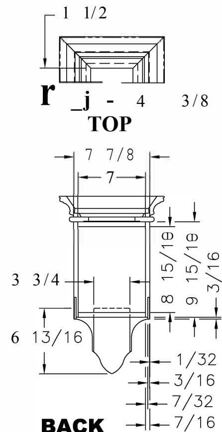
COLUMN HEADER (A) W/ HWH S/O - RH SHOWN
