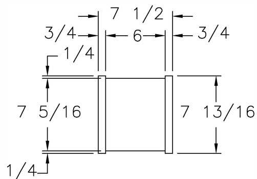
FULL WALL S-0 DIVIDER BLOCK
