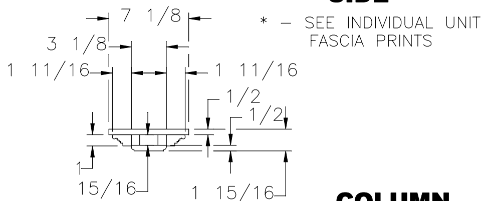
COLUMN
