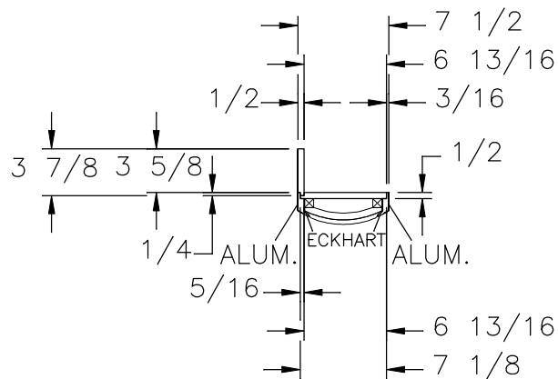
HWH NON-FLAT FLOOR VERTICAL COLUMN (RT/LT REQ'D)
