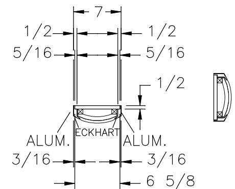
NON-HWH VERTICAL COLUMN & TYPICAL HORIZONTAL HEADER
