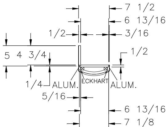
HWH FLAT FLOOR VERTICAL COLUMN (RT/LT REQ'D)
