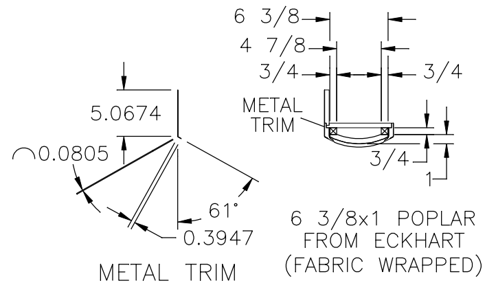
HWH NON-FLAT FLOOR VERTICAL COLUMN
