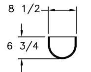
COLUMN CAP — USED W/O ADJOINING HEADER
