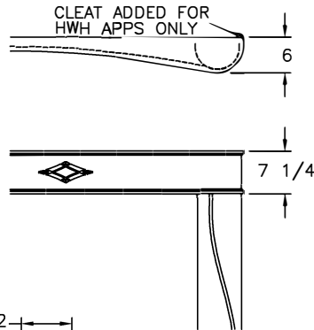
TYPICAL END LEG CONFIGURATION
