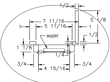
CENTER BLOCK DETAIL SECTION B-B SCALE: x4
