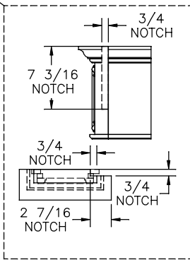
CORNER BLOCK BEDROOM W/SOFFIT ONLY
