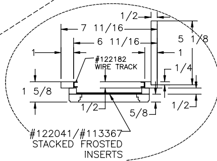
VERTICAL FASCIA DETAIL SECTION A-A SCALE: x4
