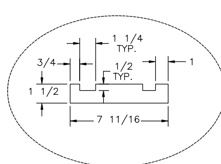
FASCIA BOTTOM CAP DETAIL SECTION D-D SCALE: x4
