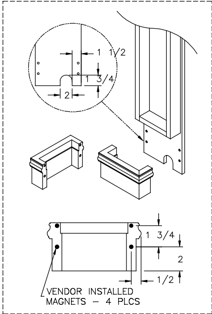
MAGNET INSTALLATION DETAIL
