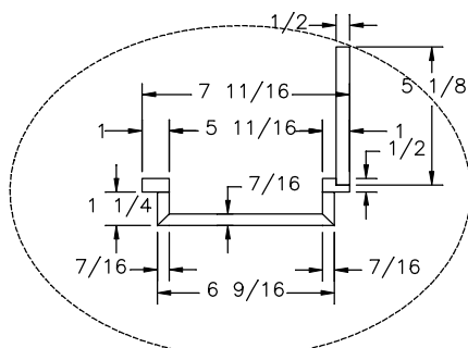
FOOT BLOCK DETAIL SECTION C-C SCALE: x4
