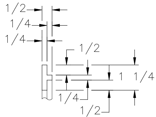
A-A (TYP. PERIMETER) (ENLARGED 4X)
