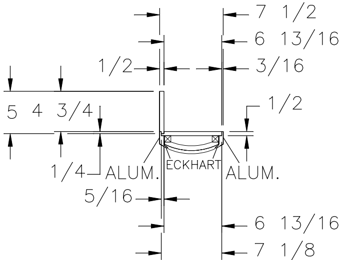
HWH FLAT FLOOR VERTICAL COLUMN (RT/LT REQ'D)
