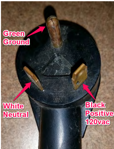
30 Amp Plug
