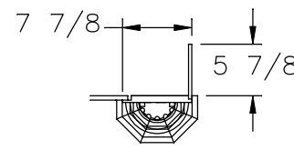
TYPICAL FLUSH FLOOR HWH COLUMN
