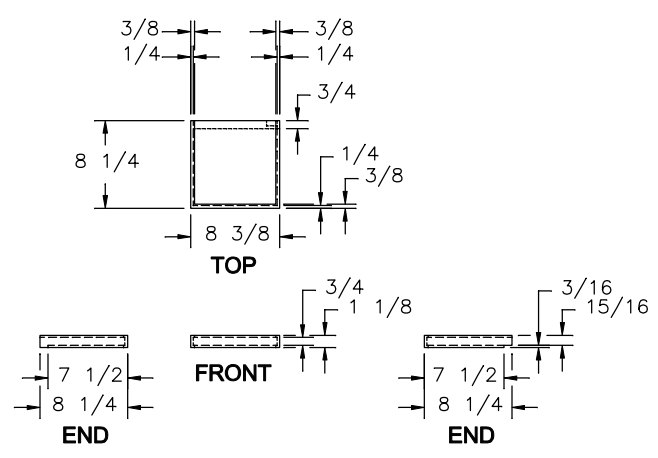
NON-HWH HEAD PIECE (LEFT/RIGHT REQ'D)
