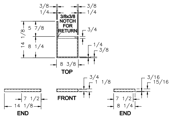
HWH FLAT FOOR HEAD PIECE (LEFT/RIGHT REQ'D)
