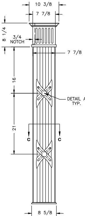
VERT COLUMN FRONT AT DRESSER
