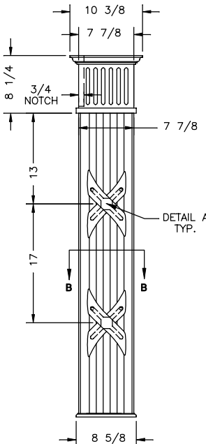
VERT COLUMN FRONT VIEW DOOR SIDE TOP OF END TABLE
