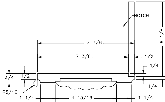
SECTION B-B SCALE X4
