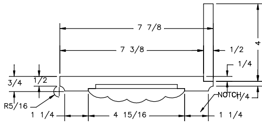
SECTION C-C SCALE X4
