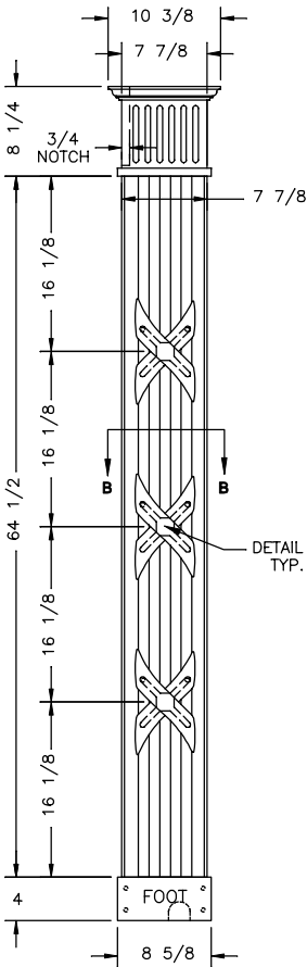
VERT COLUMN FRONT VIEW
