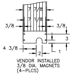
MAGNET INSTALLATION DETAIL
