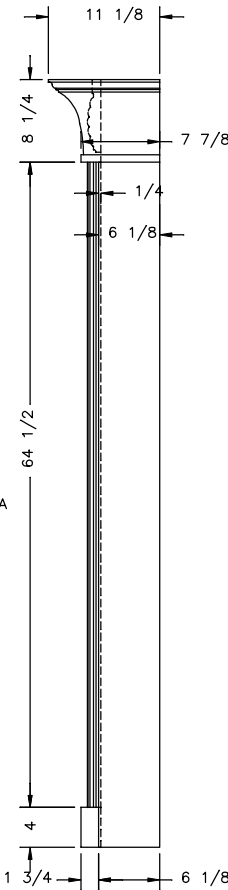
VERT COLUMN SIDE VIEW
