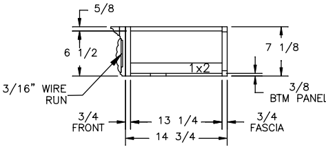
SECTION N-N
