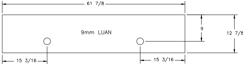
BOTTOM PANEL
