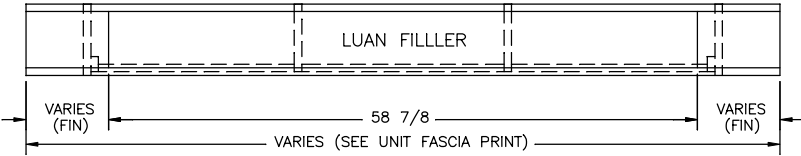
BACK VIEW
