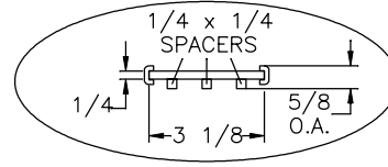
MIDDLE BOARD END VIEW SCALED 5x
