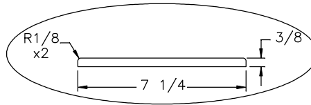
BASE BOARD END VIEW SCALED 5x
