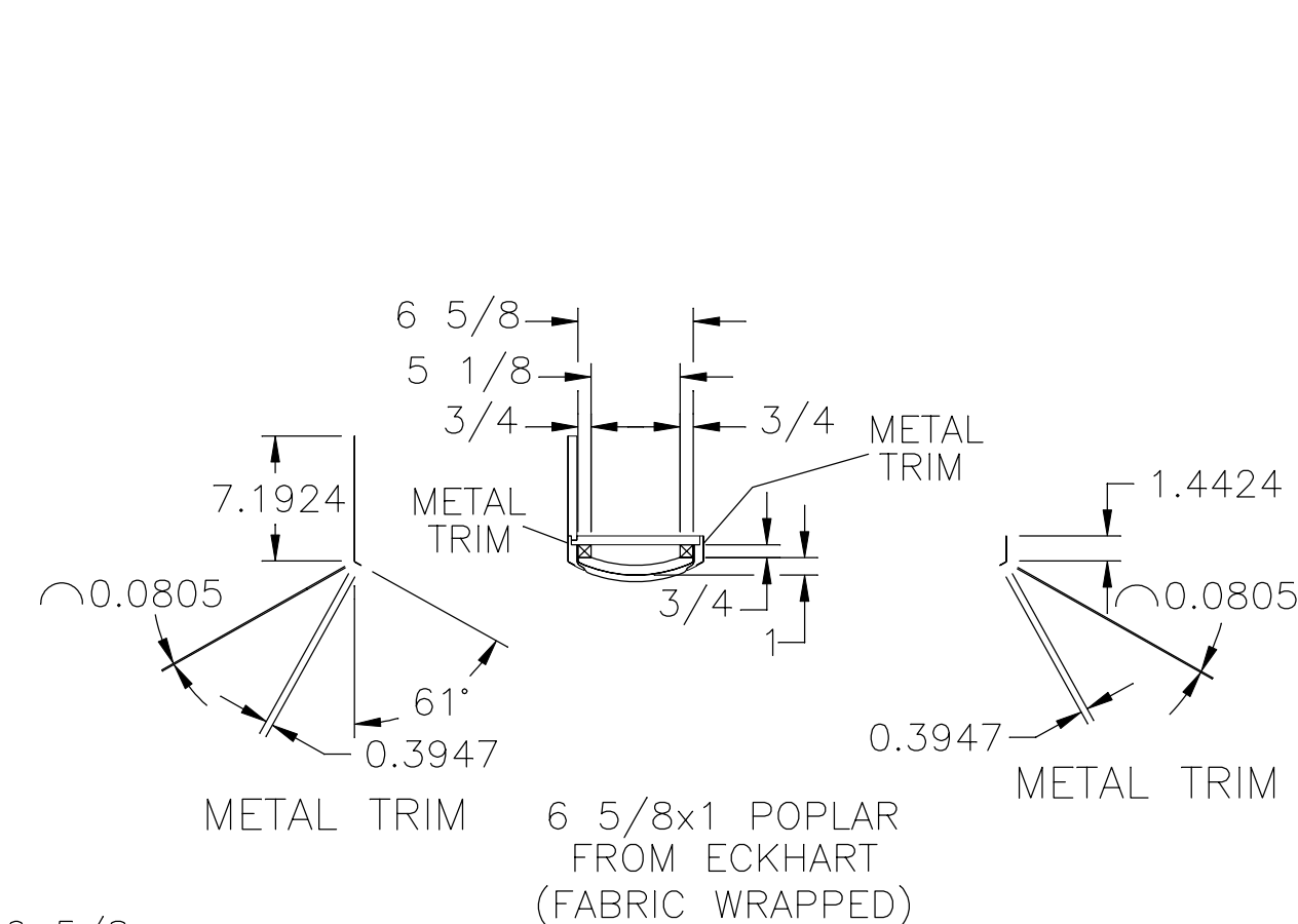
HWH FLAT FLOOR VERTICAL COLUMN
