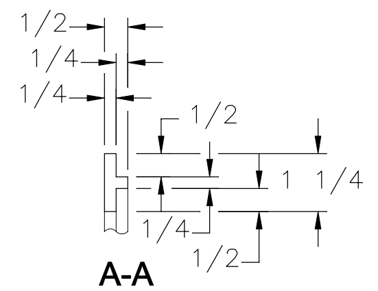
A-A (TYP. PERIMETER) (ENLARGED 4X)
