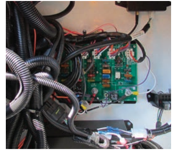
Spartan Fuse Panel Example
