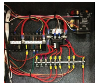
Shore Power Compartment Fuse Example
