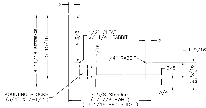
VERTICAL FASCIA SEC C-C SCALE X4
