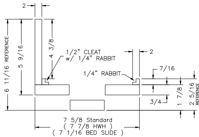
VERTICAL FASCIA SEC A-A SCALE X4
