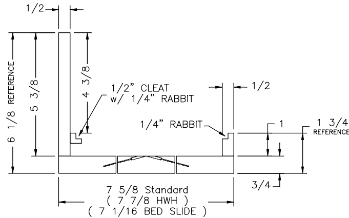
VERTICAL FASCIA SEC B-B SCALE X4
