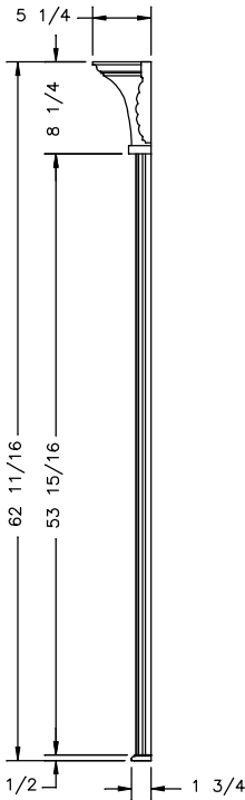
VERT COLUMN SIDE VIEW AT DRESSER
