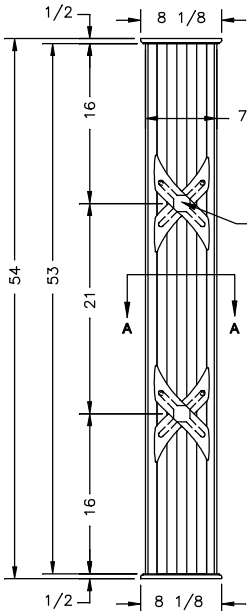
VERT COLUMN FRONT VIEW
