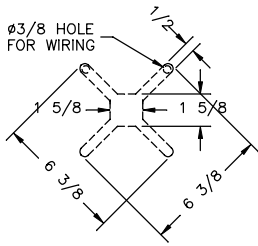
DETAIL A SCALE X2
