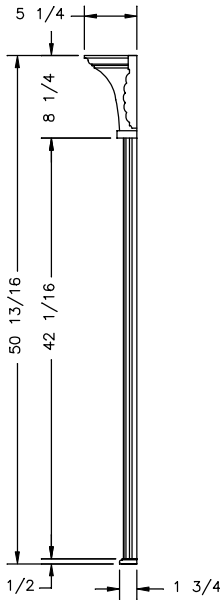
VERT COLUMN SIDE VIEW AT BED
