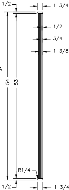
VERT COLUMN SIDE VIEW
