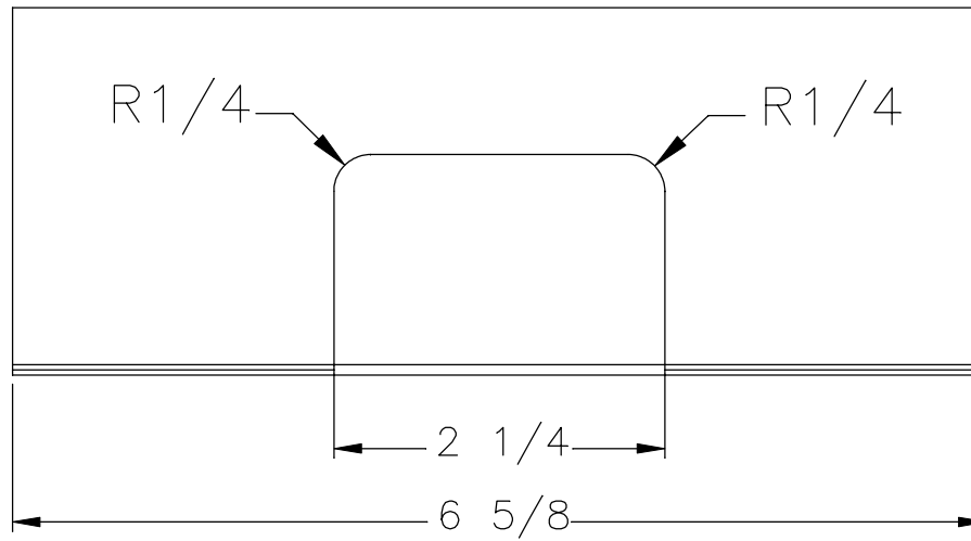
VIEW — FRONT
