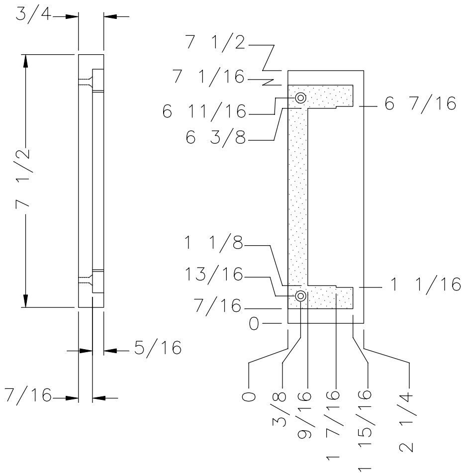
FASCIA TRIM BLOCK (DRAWN X4)
