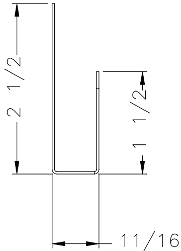
VIEW — PROFILE
