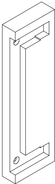
VERTICAL SPACER BLOCK (DRAWN X3)
