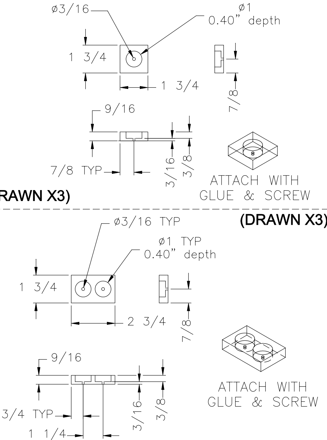
HORIZONTAL SPACER BLOCK
