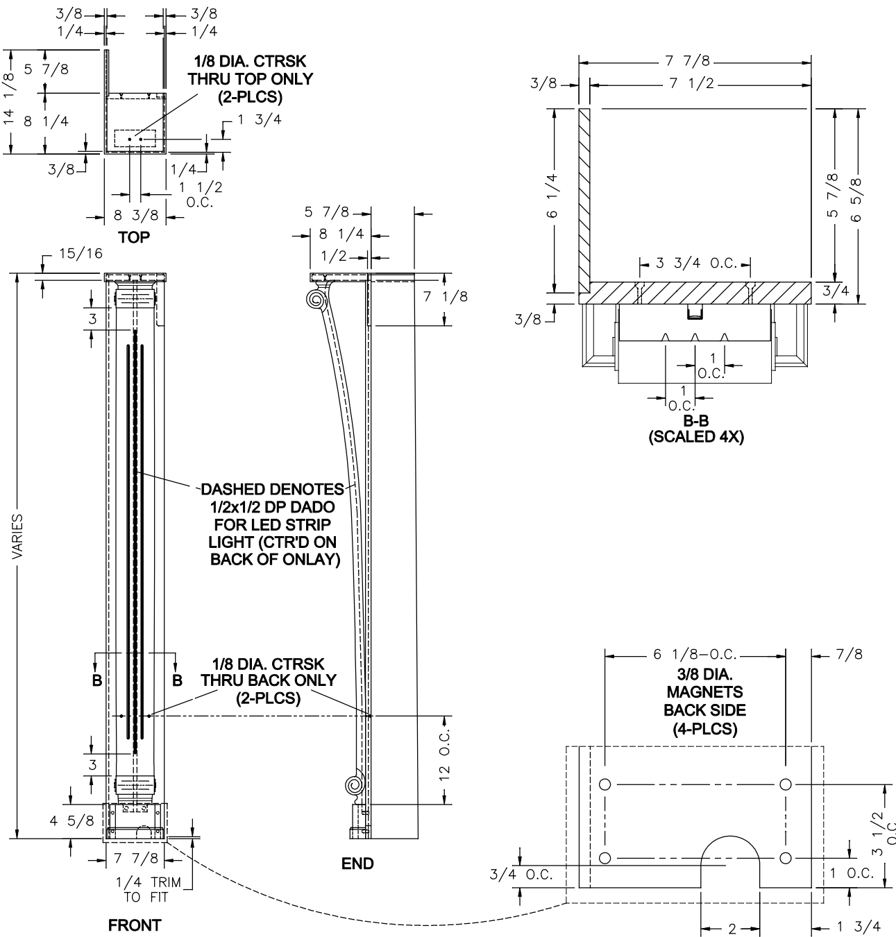
HWH FLAT FOOR COLUMN (LEFT/RIGHT REQ'D)
