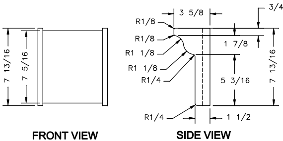
TYPICAL POCKET DOOR JAMB CONFIGURATION
