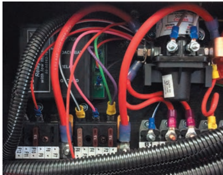
Ford Chassis Fuse Panel Example
