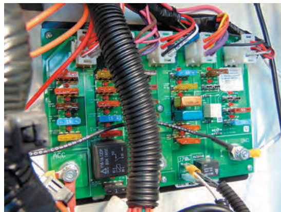
KIB Fuse Panel Example
