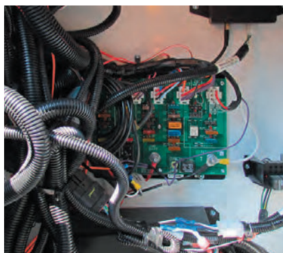
Spartan Fuse Panel Example
