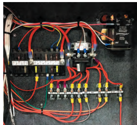
Shore Power Compartment Fuse Example
