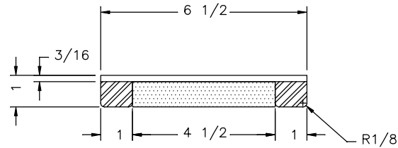
TYPICAL HORIZONTAL FASCIA BED VERTICAL FASCIA SCALE X4
