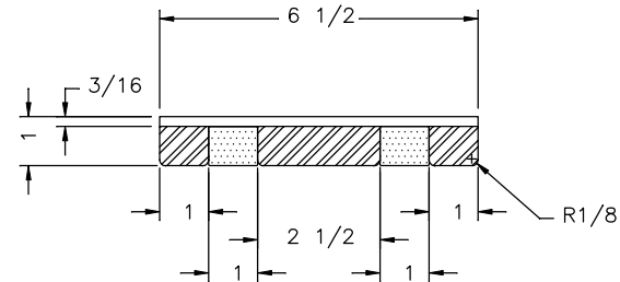
VERTICAL FASCIA BED SLIDEOUT SCALE X4
