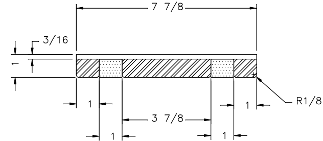
VERTICAL FASCIA HWH SLIDEOUT SCALE X4
