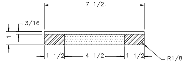
HORIZONTAL FASCIA HWH FLAT FLOOR SLIDEOUT SCALE X4
