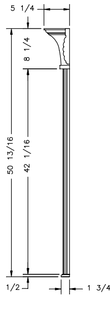
VERT COLUMN SIDE VIEW AT BED
