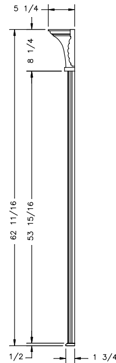
VERT COLUMN SIDE VIEW AT DRESSER
