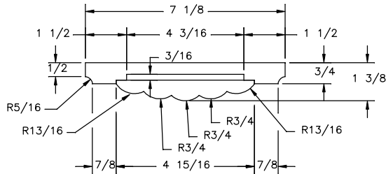
SECTION A-A SCALE X4
