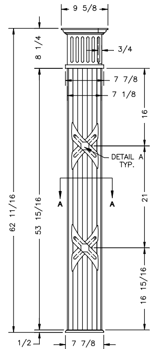
VERT COLUMN FRONT VIEW AT DRESSER
