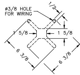
DETAIL A SCALE X2
