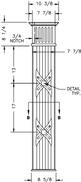
VERT COLUMN FRONT VIEW DOOR SIDE TOP OF END TABLE
