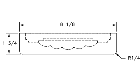
VERT COLUMN TOP VIEW AND BOTTOM VIEW SCALE X4
