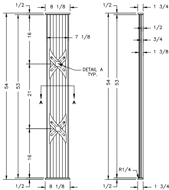
VERT COLUMN FRONT VIEW
