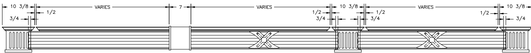
HORIZONTAL HEADER VIEW
