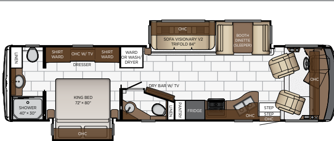
Length: 36' 11"
