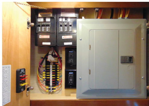
Diesel Pusher Fuse Panel Example
