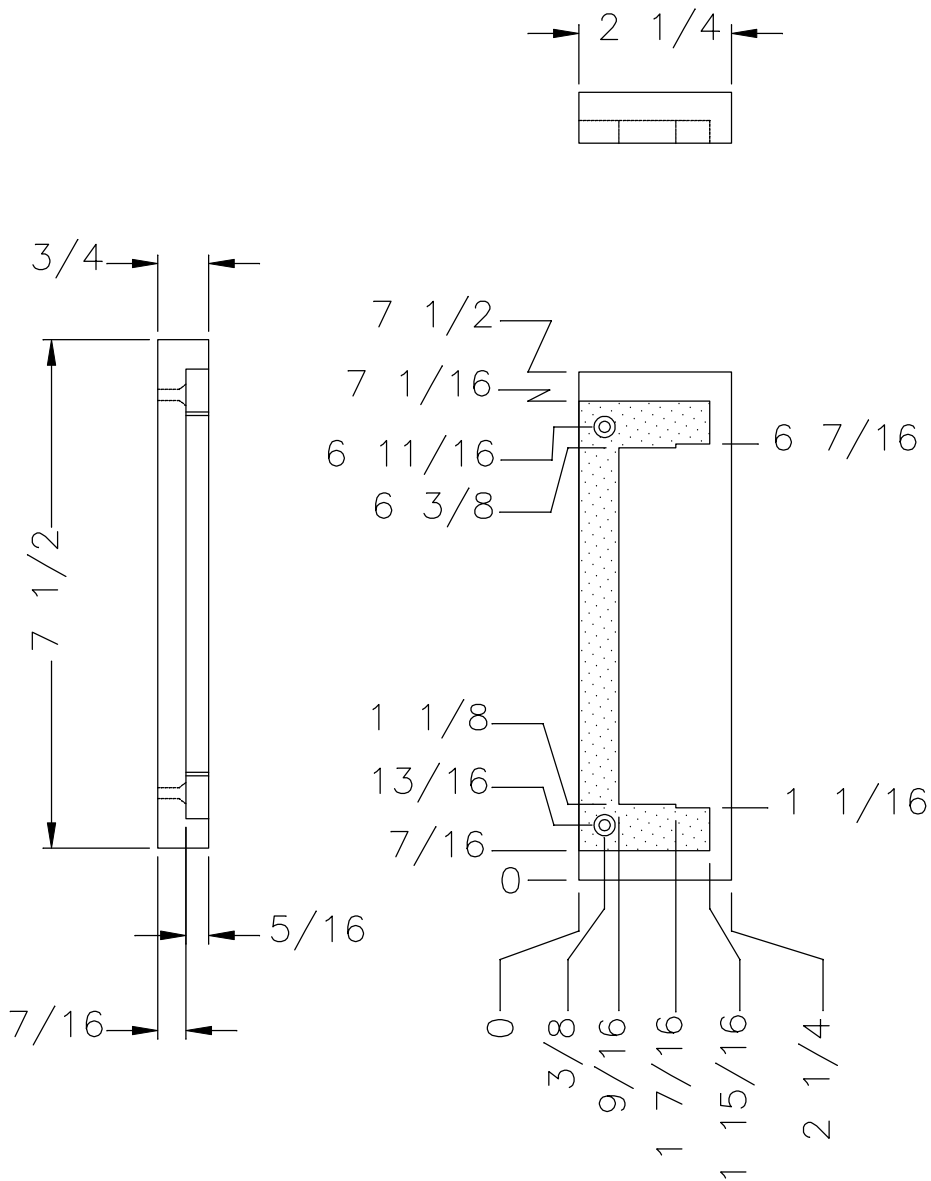
FASCIA TRIM BLOCK (DRAWN X4)
