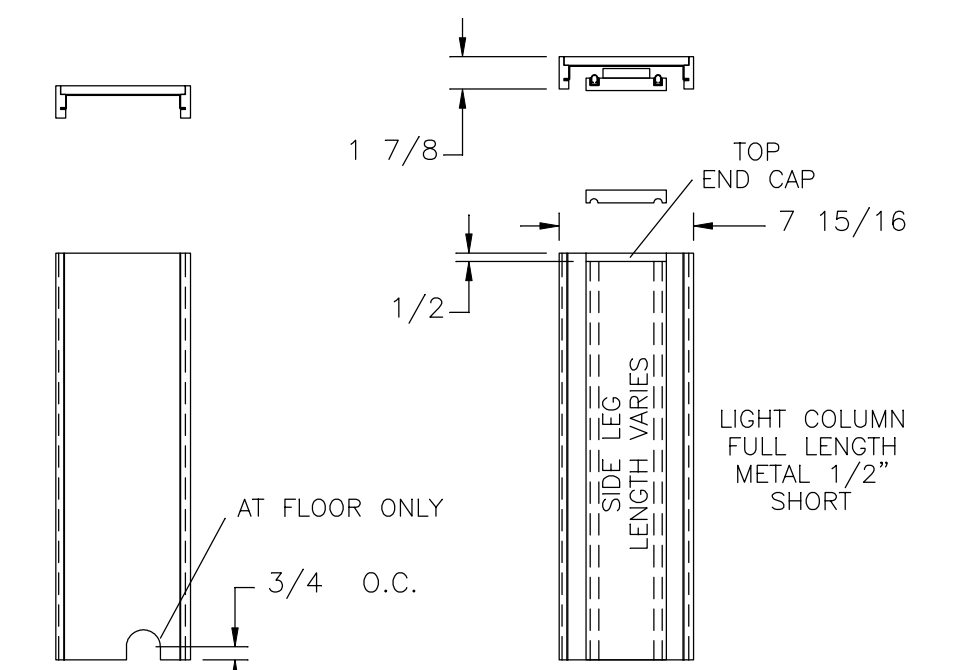
HWH VERTICAL COLUMN (RT/LT REQ'D)
