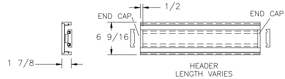
LIVINGROOM/KITCHEN HWH HORIZONTAL HEADER
