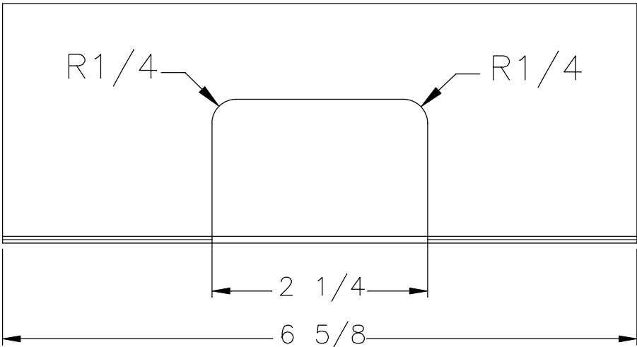
VIEW — FRONT
