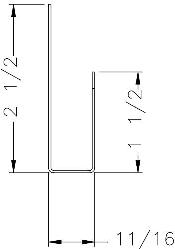
VIEW — PROFILE
