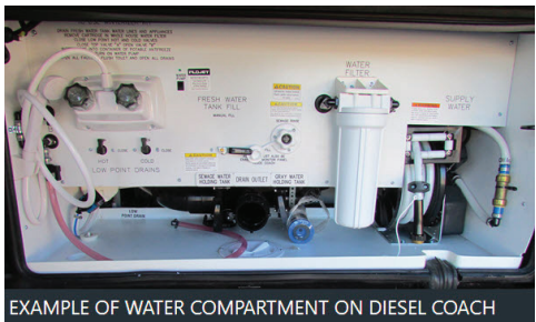
EXAMPLE OF WATER COMPARTMENT ON DIESEL COACH
