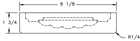
VERT COLUMN TOP VIEW AND BOTTOM VIEW SCALE X4
