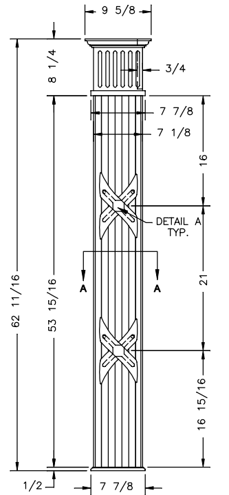
VERT COLUMN FRONT VIEW AT DRESSER
